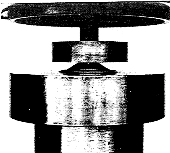
Figure 10. Photograph showing the outward flattening of frusta.
