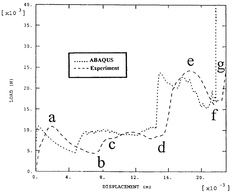
Figure 8. Experimental and FE load-displacement curves for quasi-static outward flattening of aluminum frustum.
