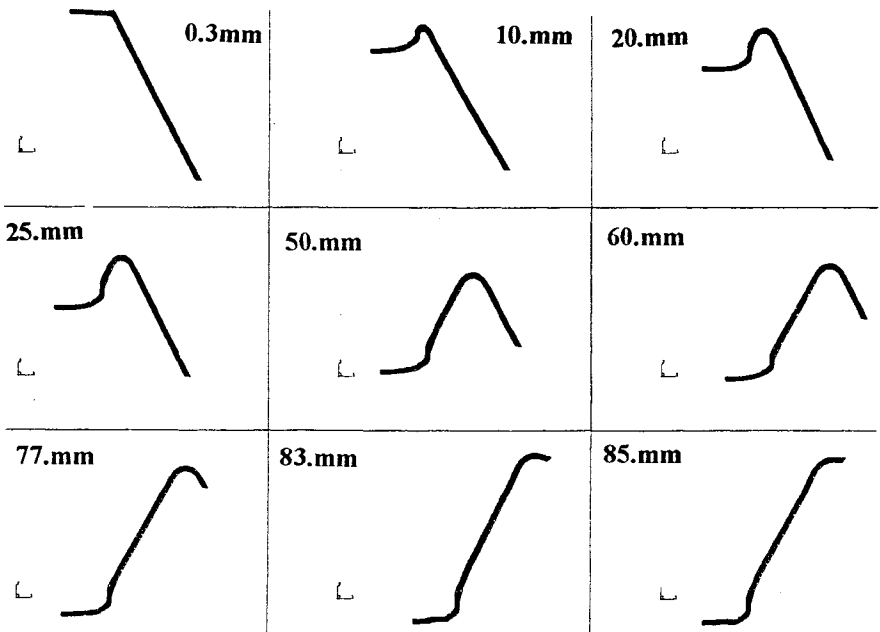
Figure 6. ABAQUS deformed plots for inward inversion of aluminum frustum.
