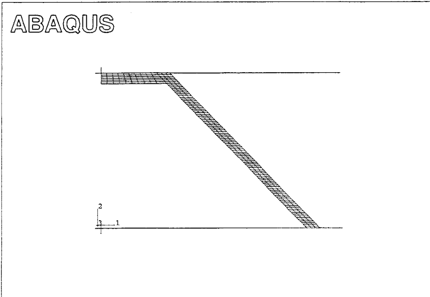
Figure 4. FE model for flattening of frusta.
