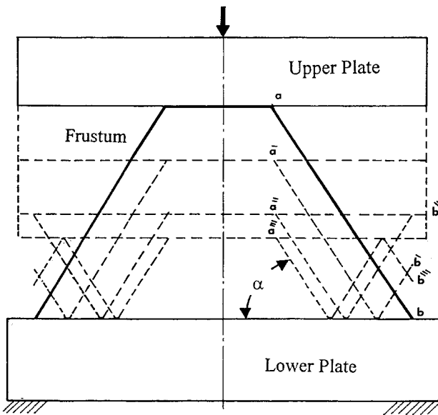
Figure 2. Outward (indirect) flattening of frusta.
