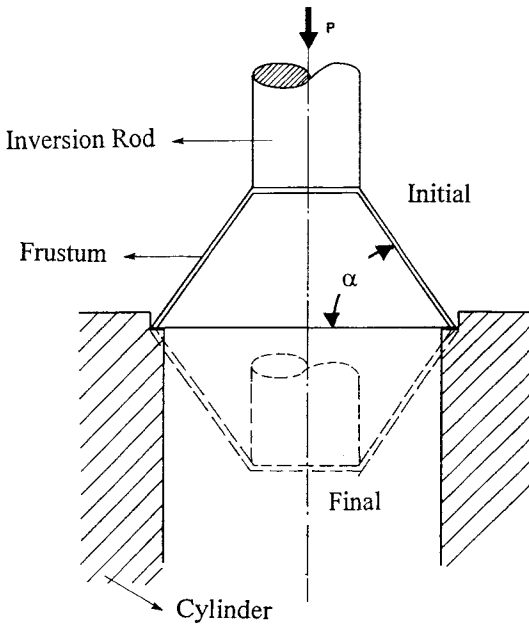
Figure 1. Inward (direct) inversion of frusta.
