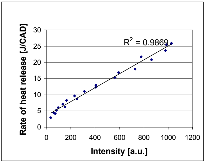
Figure 5. Variation of image average maximum intensity versus rate of heat release and linear trend line for the base case, calculated from the intensity measured horizontal through the glass liner.
