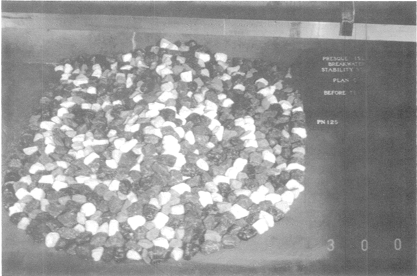
Photo 14. Long axis view of Plan C before testing with all wave conditions
