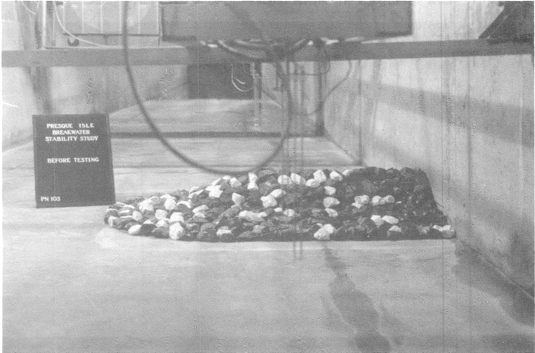
Photo 3. Beachside view of Plan A before testing with monochromatic waves
