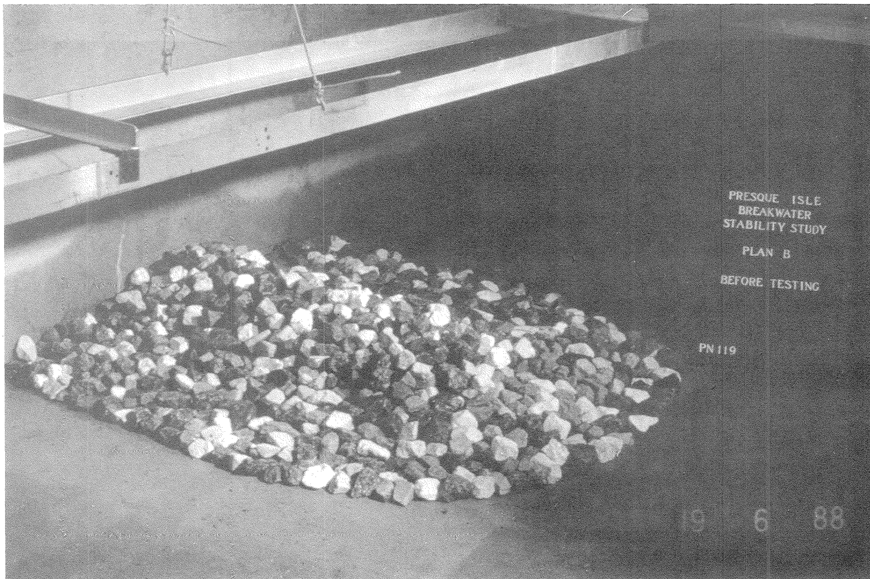
Photo 7. Lakeside view of Plan B before testing with monochromatic waves
