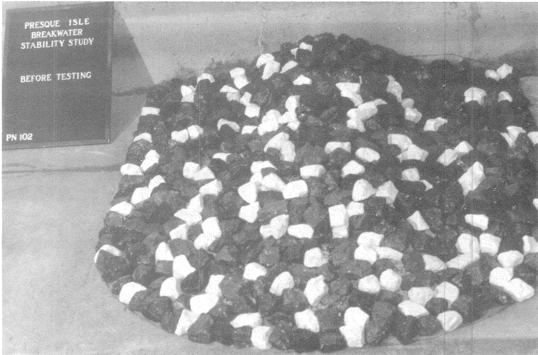
Photo 2. Long axis view of Plan A before testing with monochromatic waves
