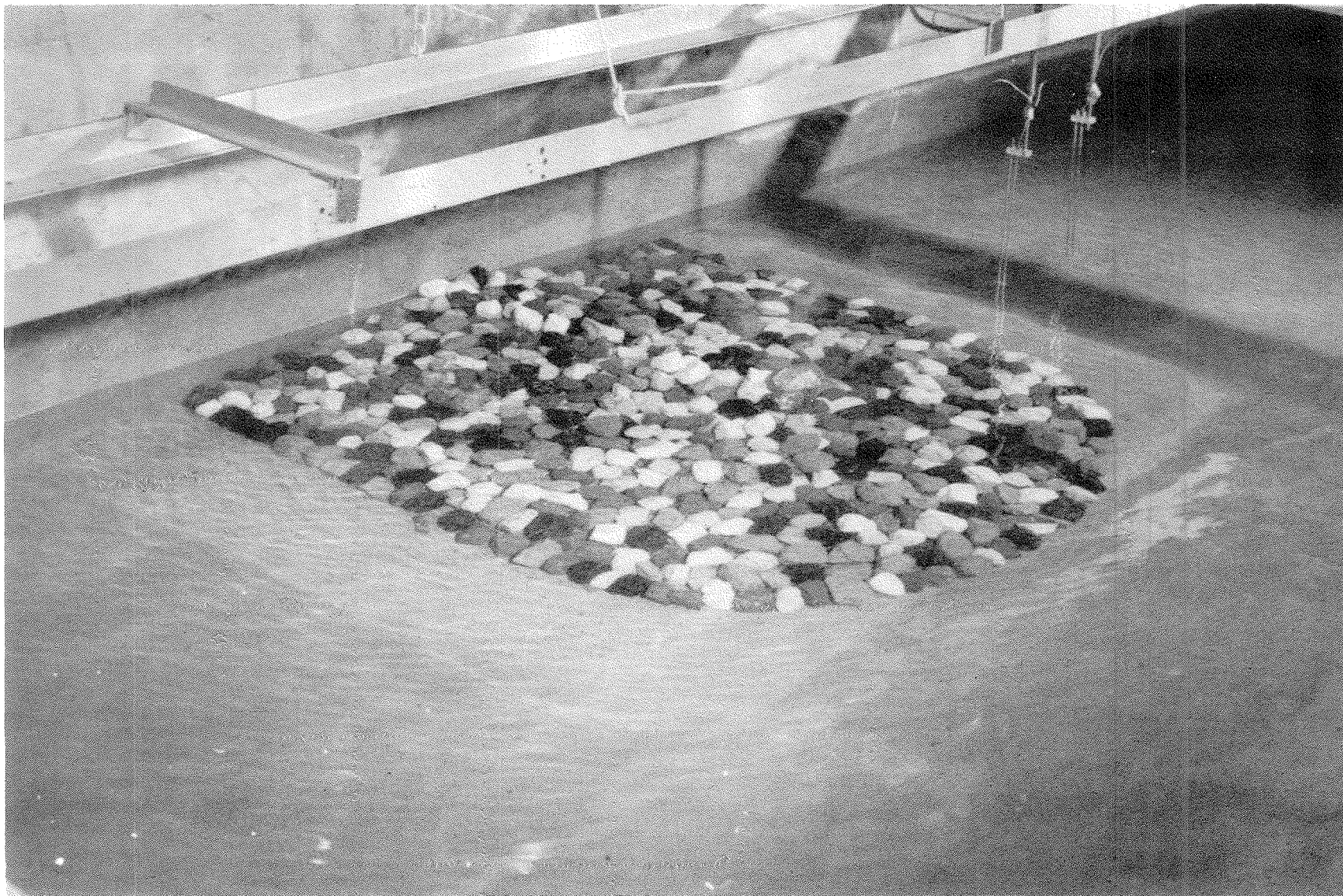
Photo 16. Lakeside view of Plan C after testing
