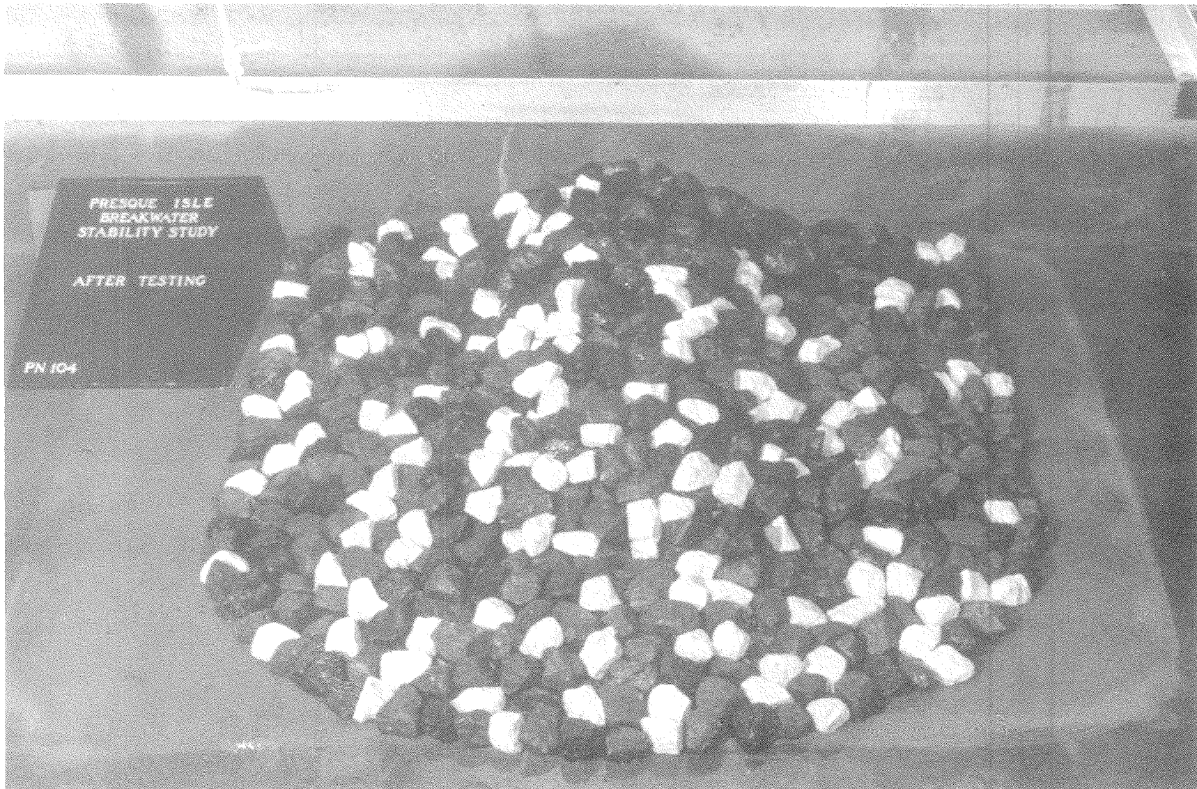
Photo 5. Long axis view of Plan A after testing with monochromatic waves
