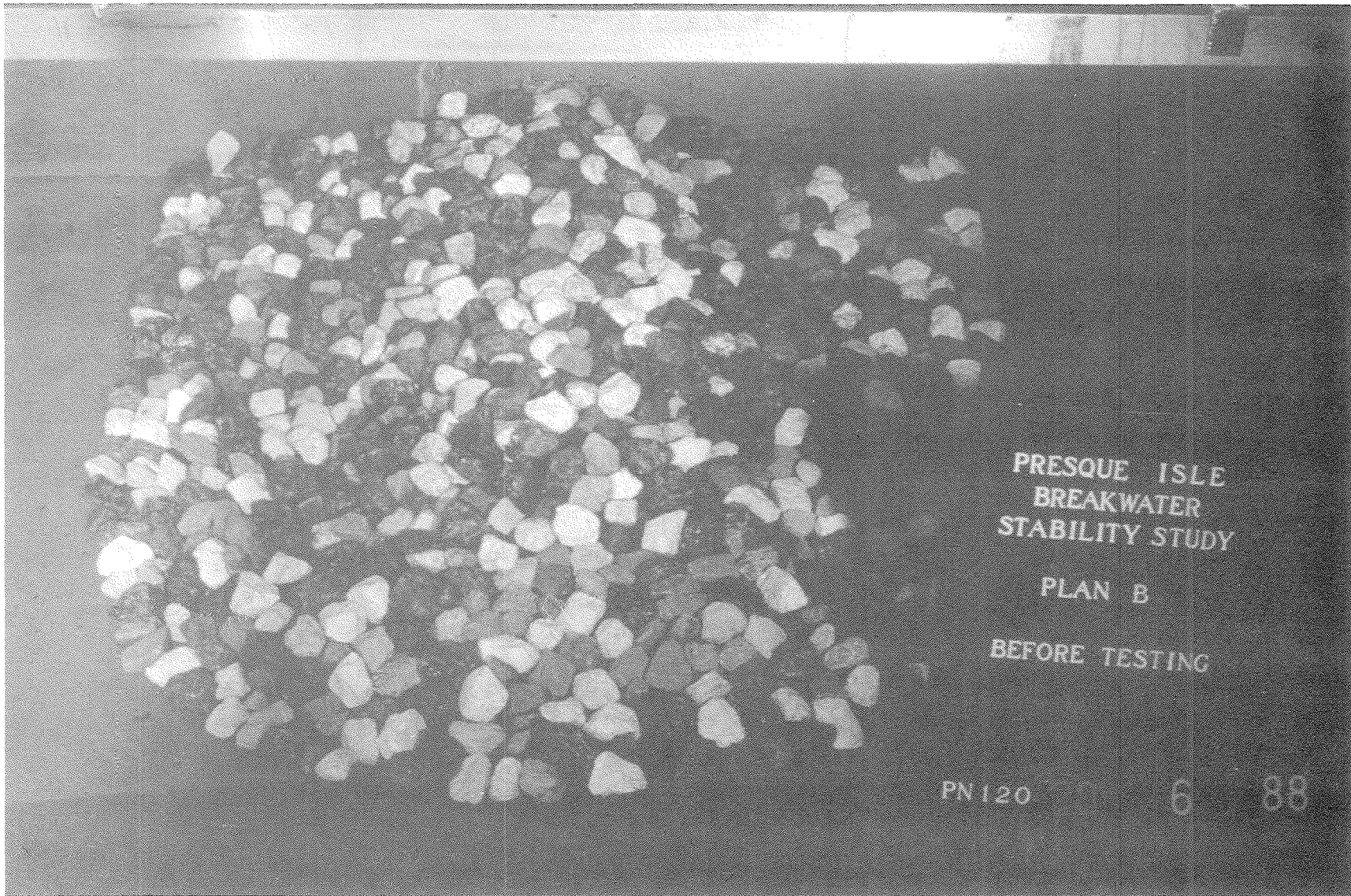
Photo 8. Long axis view of Plan B before testing with monochromatic waves
