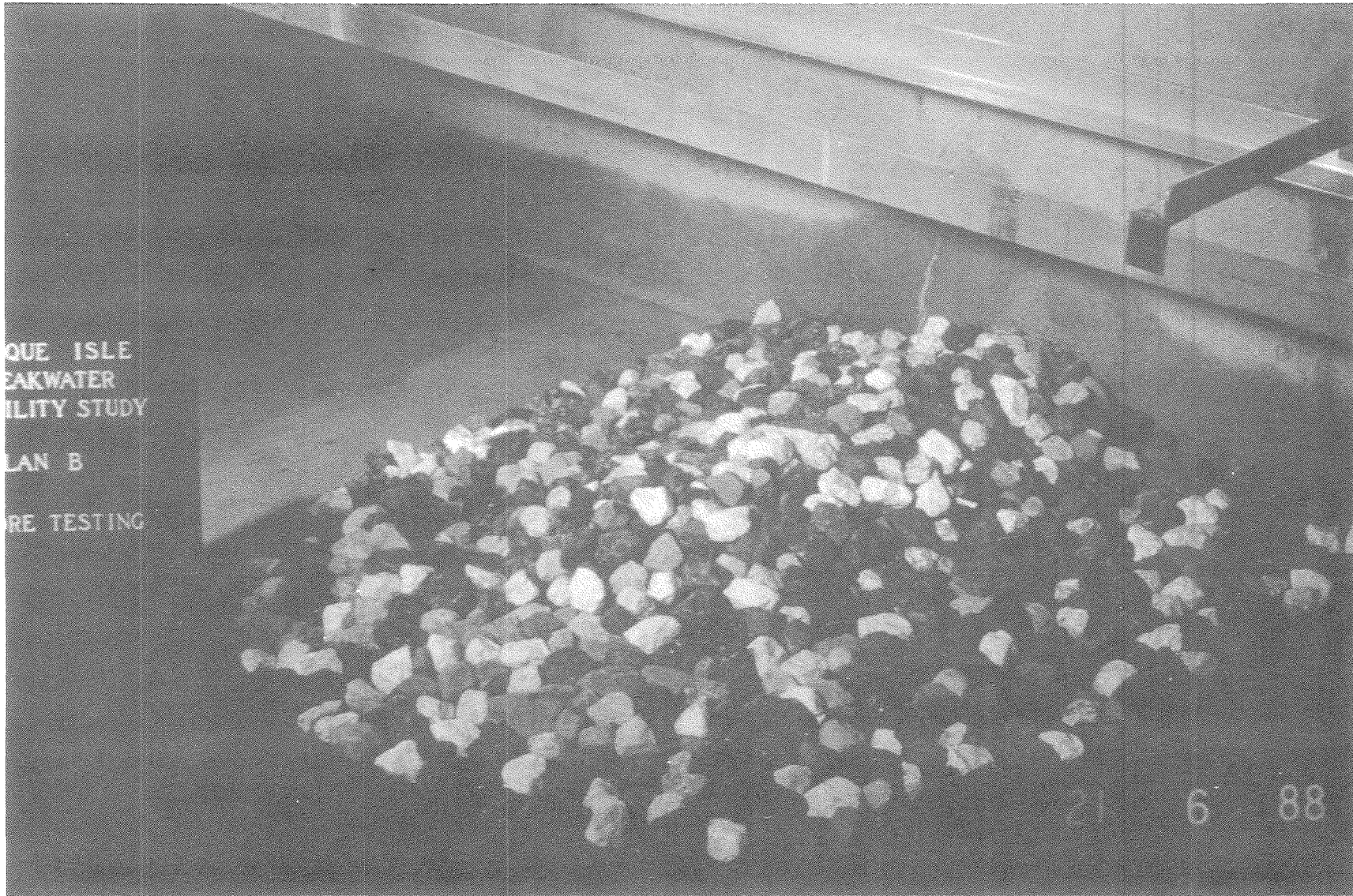
Photo 9. Beachside view of Plan B before testing with monochromatic waves
