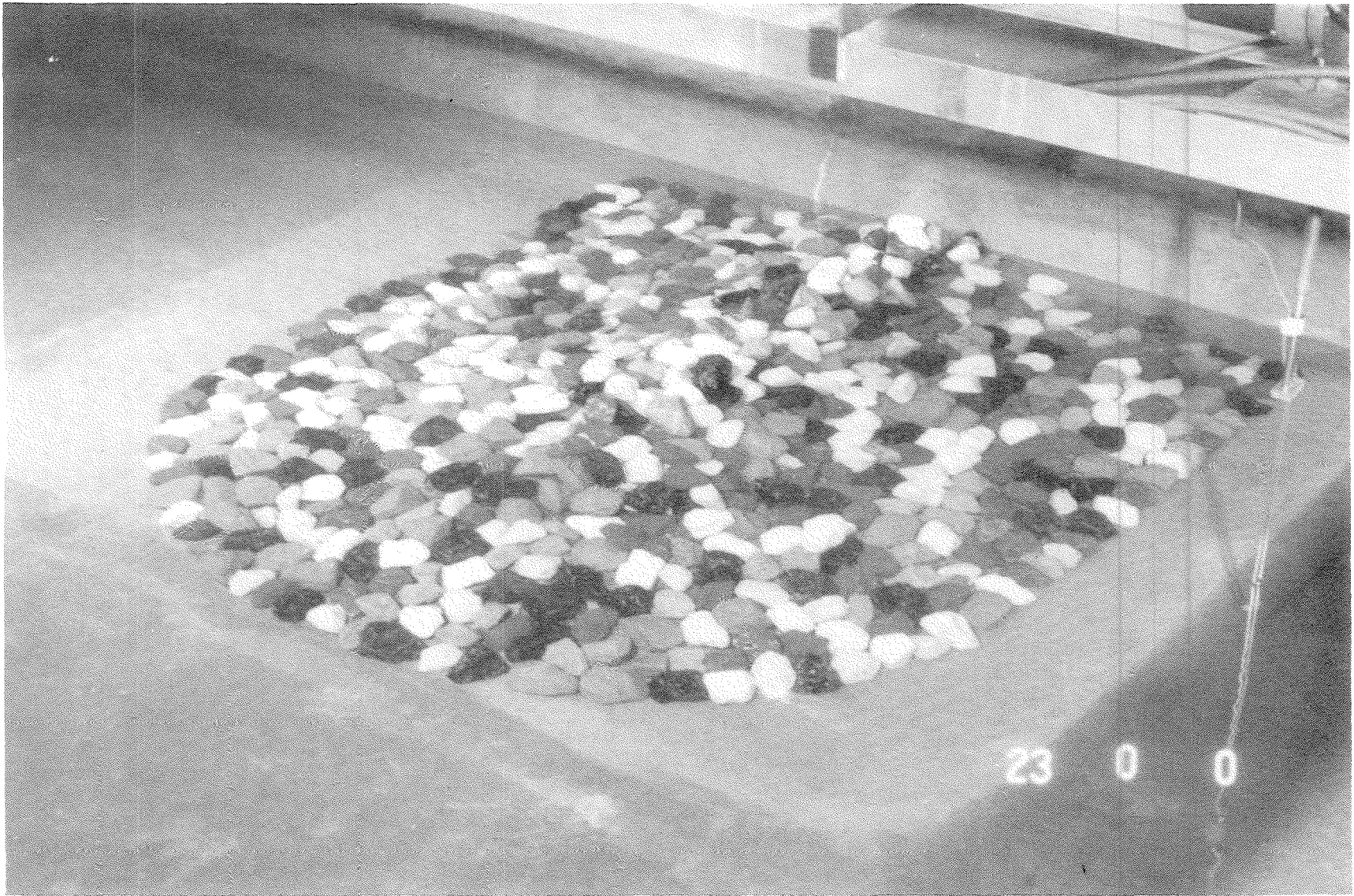
Photo 18. Beachside view of Plan C after testing
