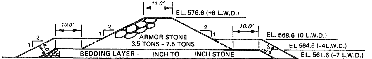
TYPICAL SECTION BEACH NO. 1 TO BEACH NO. 5 21 BREAKWATER SEGMENTS
