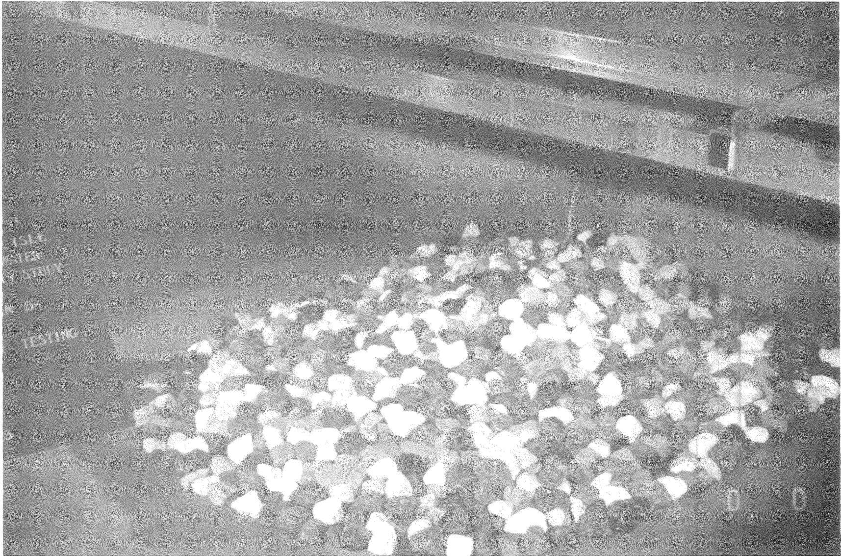
Photo 12. Beachside view of Plan B after testing with monochromatic waves
