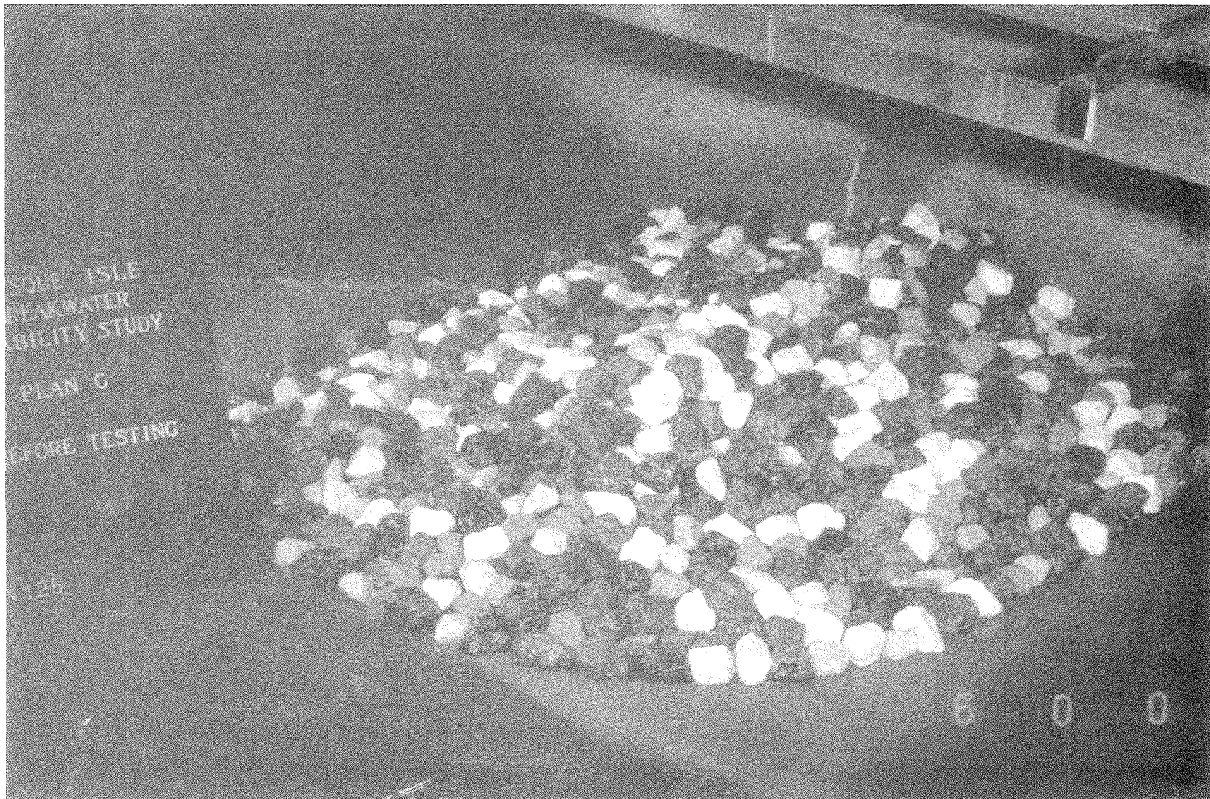
Photo 15. Beachside view of Plan C before testing with all wave conditions
