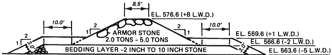
TYPICAL SECTION BEACH NO. 6 TO BEACH NO. 10 37 BREAKWATER SEGMENTS
