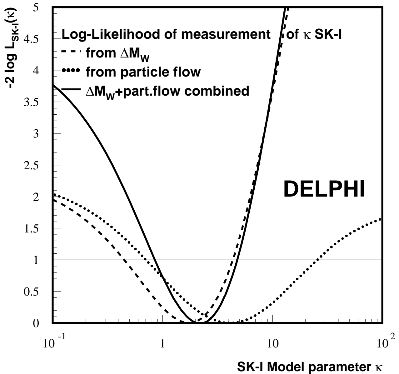
Figure 18: The log-likelihood function -2 \log L(\kappa) obtained from the combined DELPHI measurement via \Delta M_W(\text{std}, R_{\text{cone}} = 0.5 \text{ rad}) and the particle flow. The full line gives the final result including the statistical and systematic uncertainties. The log-likelihood functions are combined in the hypothesis of no correlation between the statistical and systematic uncertainties of both measurements.
