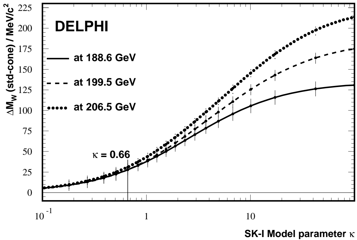
Figure 15: The dependence of the observable \Delta M_W(\text{std}, R_{\text{cone}} = 0.5 \text{ rad}) from simulation events on the value of the SK-I model parameter \kappa . The dependence is given at three centre-of-mass energies.
