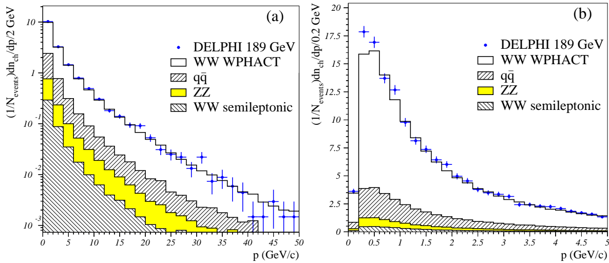
Figure 1: Momentum distribution for charged particles (range 0-50 GeV/c (a) and 0-5 GeV/c (b)). Points represent the data and the histograms represent the contributions from simulation for the different processes (signal (white) and background contributions).
