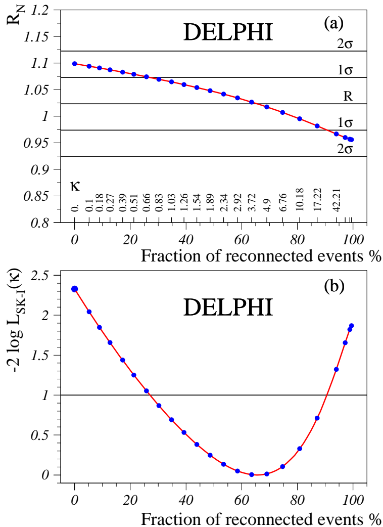
Figure 10: a) Estimated ratio R_N at 200 GeV plotted as a function of different \kappa values (top scale), or as function of the corresponding reconnection probabilities (bottom scale), compared to \langle R \rangle measured from data after rescaling to 200 GeV (horizontal lines marked with R for the value and with 1\sigma(2\sigma) for the \langle R \rangle value added/subtracted by one(two) standard deviations); the last three marks on the x axis, close to 100% of reconnection probability, correspond respectively to the values \kappa = 100, 300, 800 ; b) corresponding log-likelihood curve for the comparison of the estimated values ( R_N ) with the data ( \langle R \rangle ).
