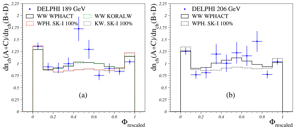
Figure 6: The ratio of the particle flow distributions (A+C)/(B+D) at 189 GeV (a) and at 206 GeV (b). The data (dots) are compared to WW MC samples generated with WPHACT (DELPHI samples) and KORALW (Cetraro samples), both without CR and implementing the SK-I model with 100% probability of reconnection. The lines corresponding to WPHACT are hardly distinguishable from the lines corresponding to KORALW in the same condition of implementation of CR.
