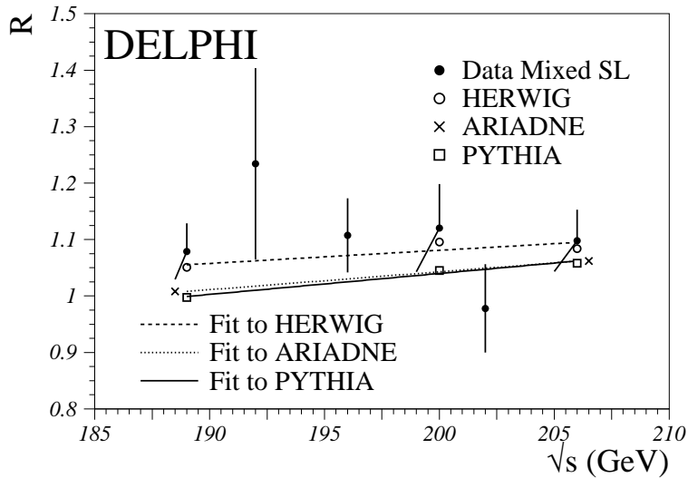
Figure 8: The ratio R_{\text{mixedSL}} as function of \sqrt{s} for data and MC, and fits to the MC (see text). The ARIADNE points at 189 GeV and at 206 GeV have their centre-of-mass energy shifted and the error bars on data are tilted for readability.
