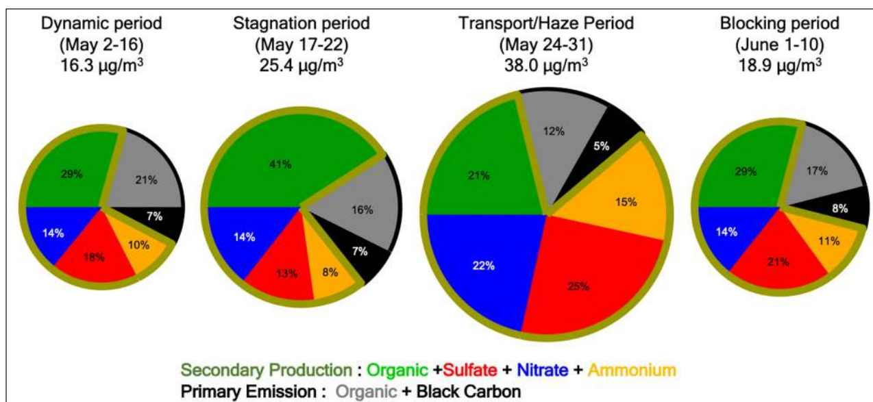
Figure 8: Mean PM 1 composition observed at the KIST ground site in Seoul for each of the 4 meteorological periods during KORUS-AQ. The size of the pie charts is scaled to the total mean aerosol concentration of the period. The outer black arc on each pie signifies primary aerosols, while the green outline encompasses secondary aerosols. DOI: https://doi.org/10.1525/elementa.424.f8
