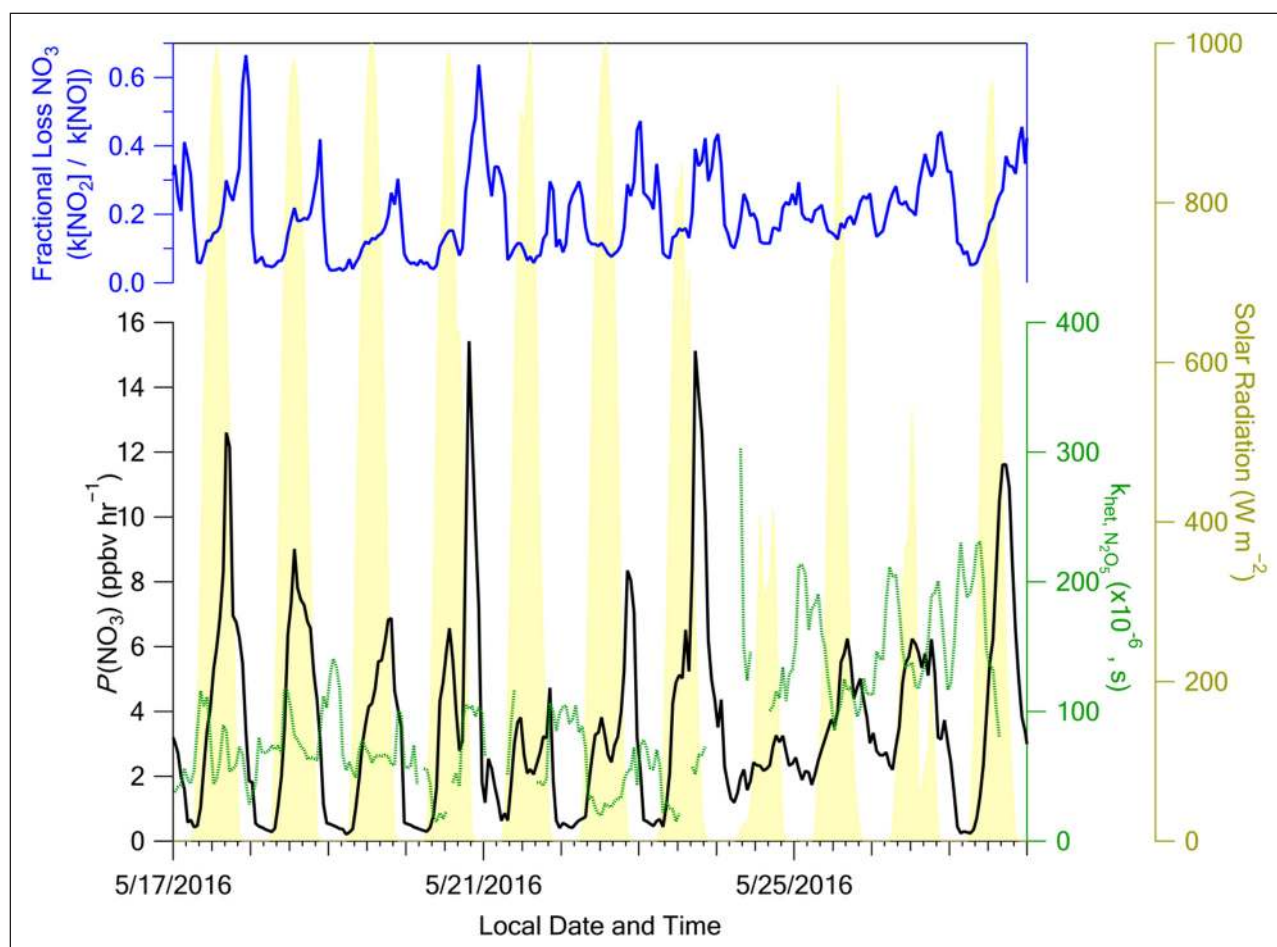
Figure 13: Top blue curve: fraction of the NO_3 radical lost via its reaction with NO_2 (reaction R3 in text) versus NO (reaction R6 in text). Lower black curve: production of the NO_3 radical ( P(NO_3) ) in ppbv/hr. Lower dotted green curve: heterogeneous reaction rate of N_2O_5 . Shaded yellow curve: solar radiation ( W/m^2 ). DOI: https://doi.org/10.1525/elementa.424.f13
