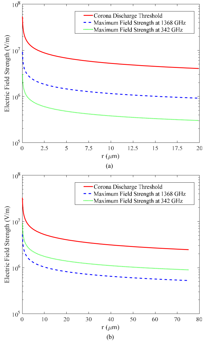
Fig. 7. Variations of the maximum electric field strengths at the designed frequencies and the corona discharge thresholds as functions of r : (a) for the high-pass FSS; (b) for the low-pass one.
