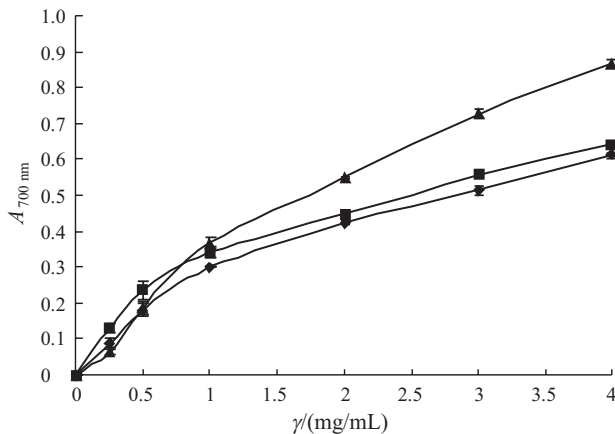
Fig. 2. Reducing power of three series of gelatin polypeptides as a function of the used concentrations. (◆) SCP1, (■) SCP2, (▲) SCP3. Bars indicate the standard deviation of triplicate determinations
