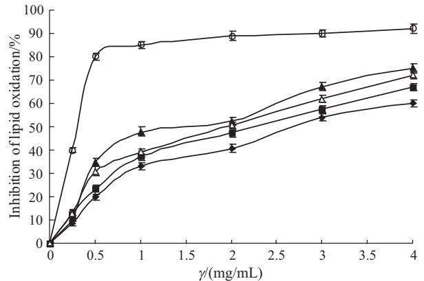
Fig. 3. Antioxidant activity of three series of gelatin polypeptides, butylated hydroxytoluene (BHT) and \alpha -tocopherol as a function of concentrations used. (◆) SCP1, (■) SCP2, (▲) SCP3, (○) BHT, (△) \alpha -tocopherol. Bars indicate the standard deviation of triplicate determinations
