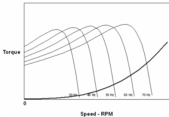
Figure 10 Torque-speed characteristics of induction motors operating with VFDs
