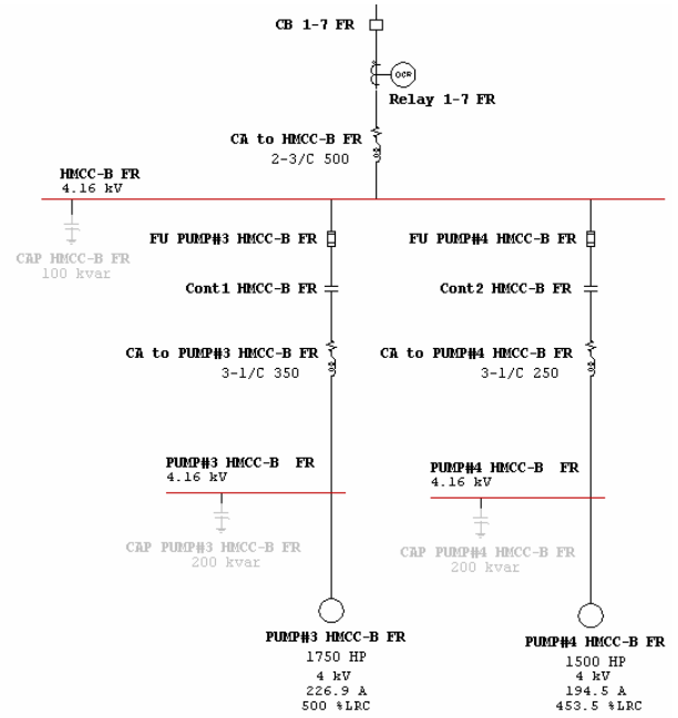
Figure 2 Single-line diagram of the 4.16KV motor control center with two water injection pumps
