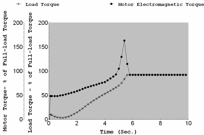
Figure 3 Load torque and motor electromagnetic torque during the motor starting for 1750HP water injection pump
