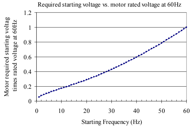
Figure 8 Required starting voltage times the motor rated voltage at 60Hz as a function of the starting frequency of VFDs
