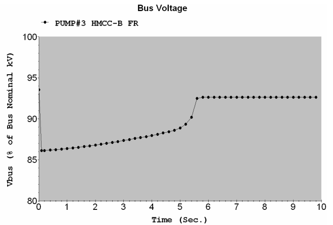
Figure 6 Voltage at the MCC main bus, HMCC-B FR
