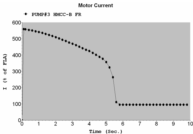
Figure 5 Motor starting current for the 1750HP water injection pump
