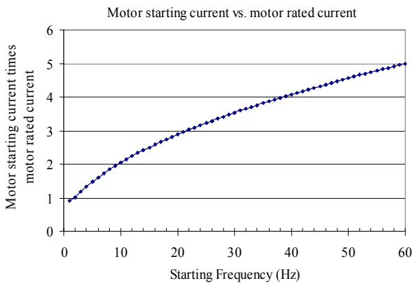
Figure 7 Motor starting current times rated current as a function of the starting frequency of VFDs
