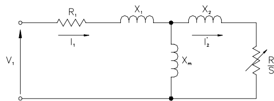
Figure 1 Equivalent circuit of Induction motors
