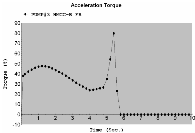
Figure 4 Acceleration torque during the motor starting for 1750HP water injection pump
