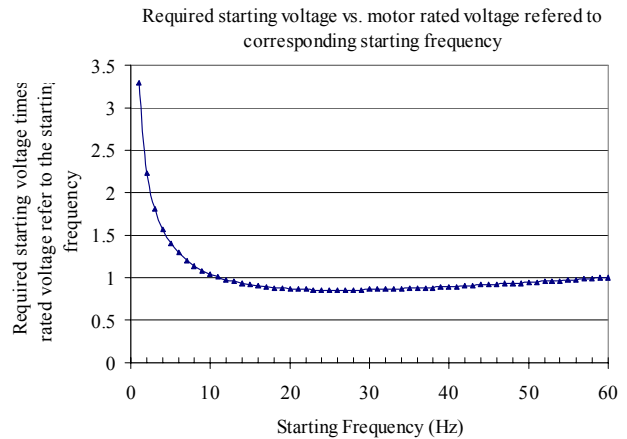
Figure 9 Required starting voltage times converted motor rated voltage from 60Hz to starting frequency as a function of starting frequency of VFDs
