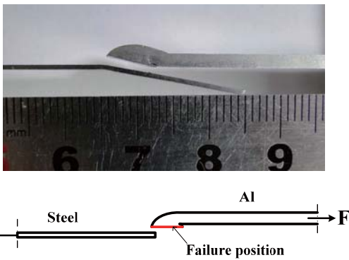
Fig. 4 Interface failure mode of CMT brazed lap joint.
