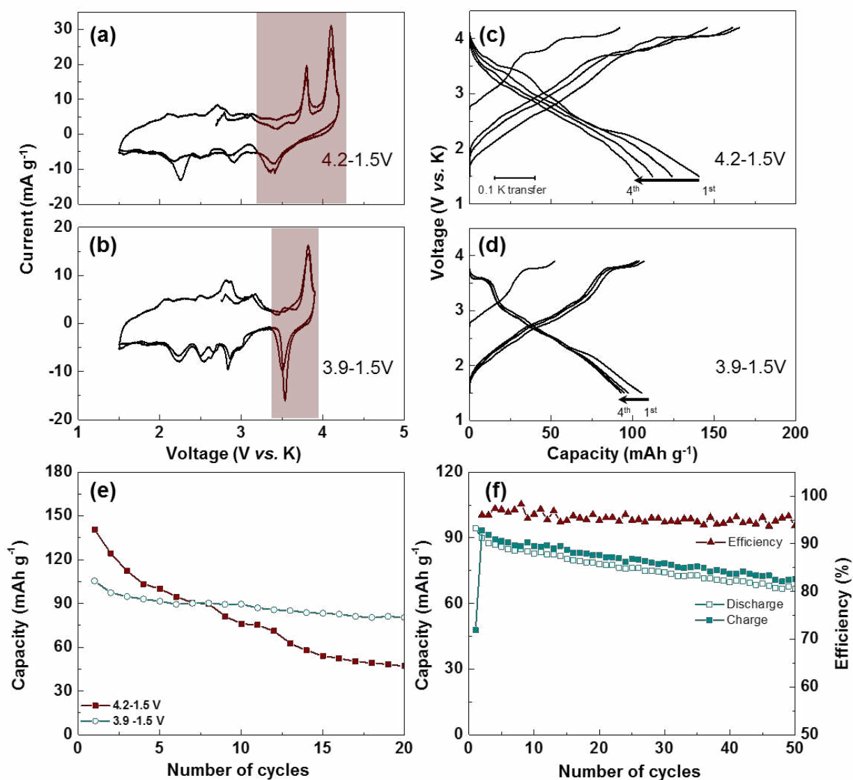
Figure 2. K-storage properties of P3- \text{K}_{0.5}\text{MnO}_2 . (a–b) Cyclic voltammograms and (c–d) galvanostatic voltage–capacity profiles of P3-type \text{K}_{0.5}\text{MnO}_2 with two different voltage cutoffs. (e) Discharge capacity of P3-type \text{K}_{0.5}\text{MnO}_2 over 20 cycles with the two different voltage cutoffs at a current rate of 5 \text{ mA g}^{-1} . (f) Cycle stability and coulombic efficiency (of the 1 st discharge) of P3-type \text{K}_{0.5}\text{MnO}_2 at a current rate of 20 \text{ mA g}^{-1} in the range of 3.9–1.5 V (vs. \text{K}/\text{K}^+ ).
