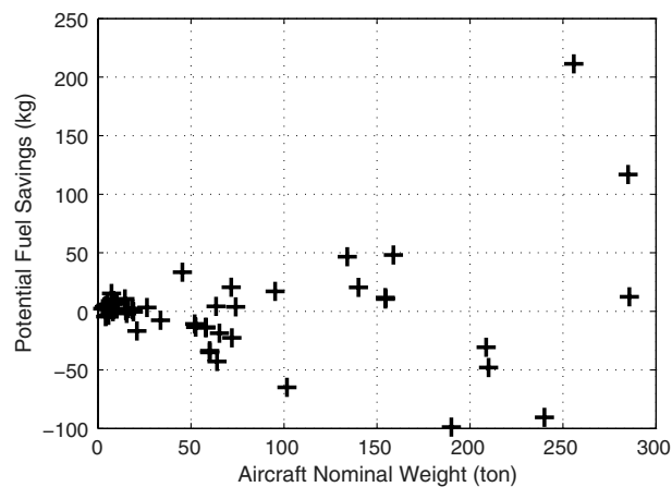
Fig. 10 Relationship between potential fuel savings and nominal weight.
