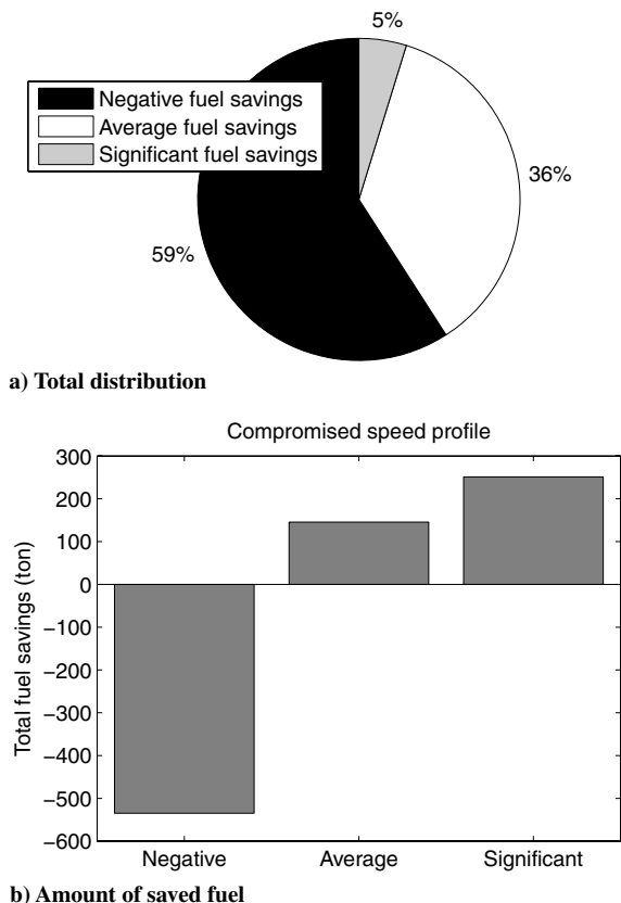
Fig. 9 Distribution of fuel consumption associated with the compromised speed profile.
