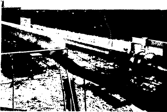
Fig. 11. Photograph of shock tube with the double diaphragm (interstage) section in the right foreground.
