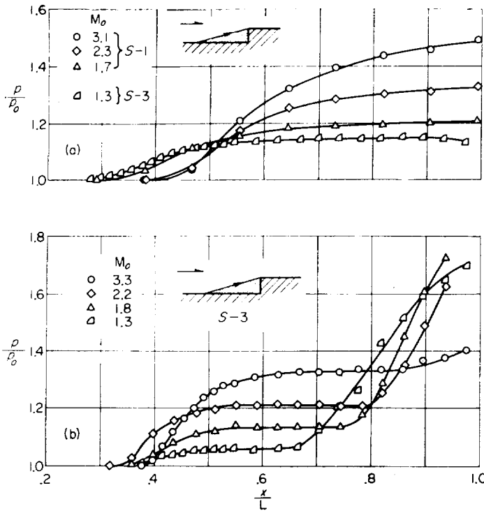
(a) Pure laminar separation; R_L \approx 0.13 \times 10^6 . (b) Transitional separation; R_L \approx 0.60 \times 10^6 .
