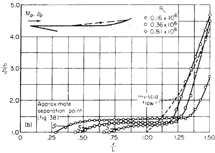
(b) Transitional separation; CS25°-1; M_0=2.7 .
