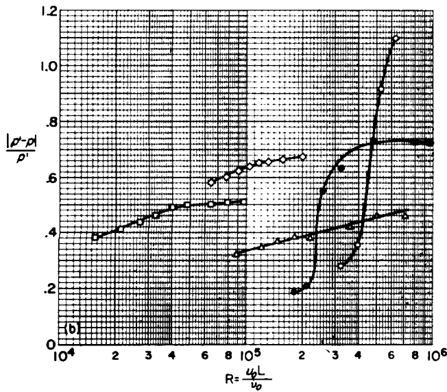
(b) Transitional separation.
