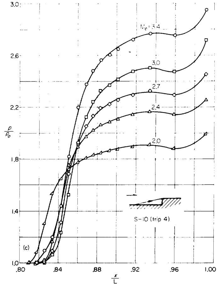
(c) Turbulent separation; R_L \approx 2.6 \times 10^6 .
