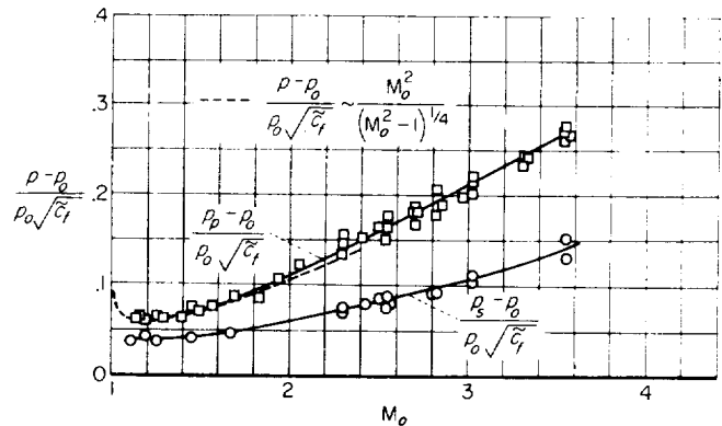
FIGURE 38.—Effect of Mach number on characteristics of laminar separation for a series of model configurations and Reynolds numbers.
