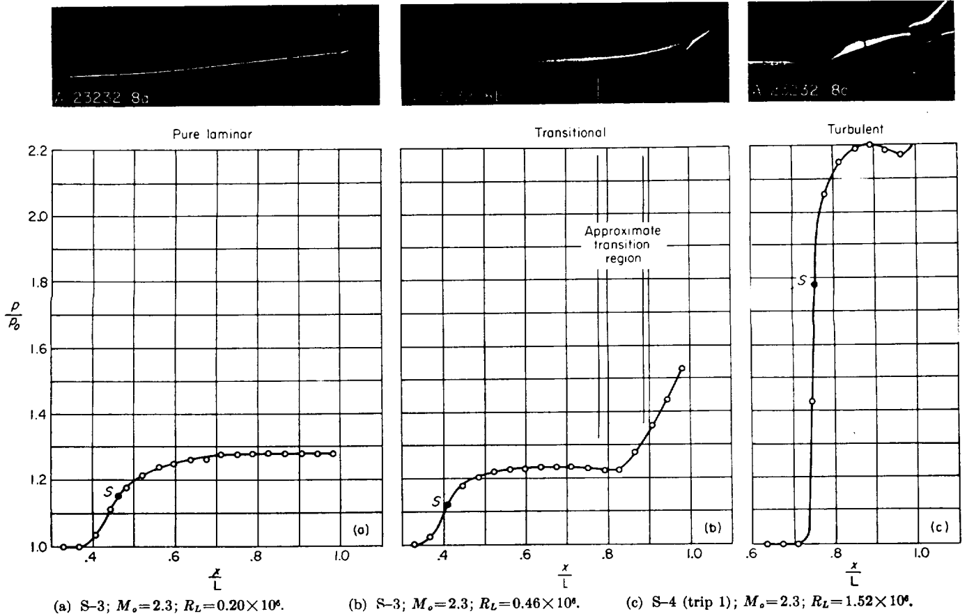
FIGURE 11.—The three regimes for a step; M_0=2.3 .
