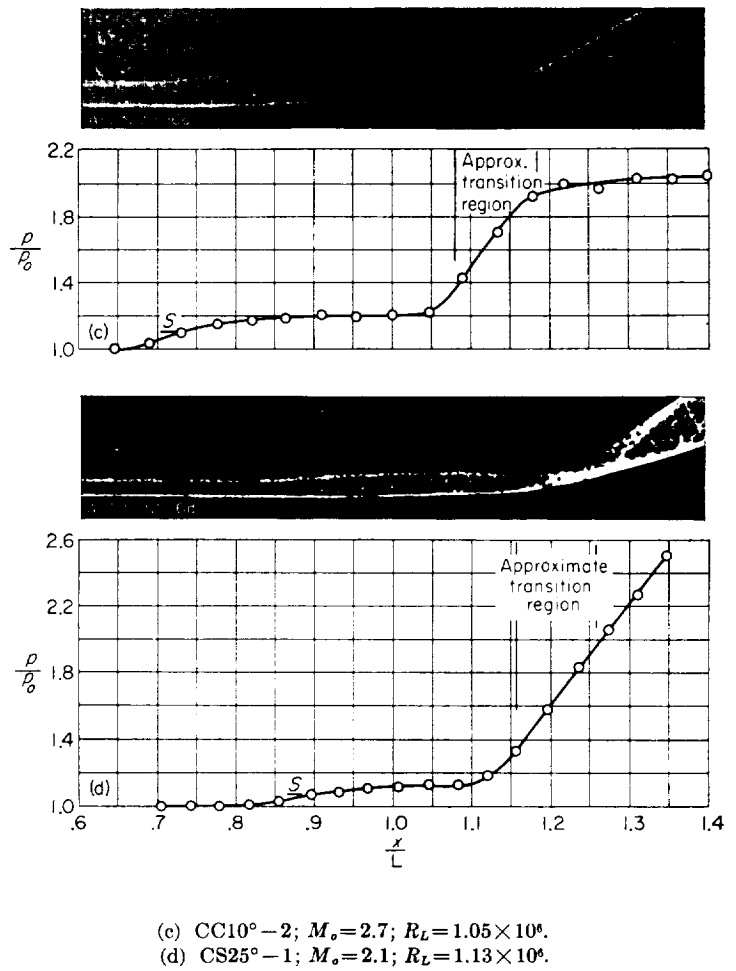
FIGURE 9.—Correlation of transition with abrupt pressure rise; high tunnel pressures.
