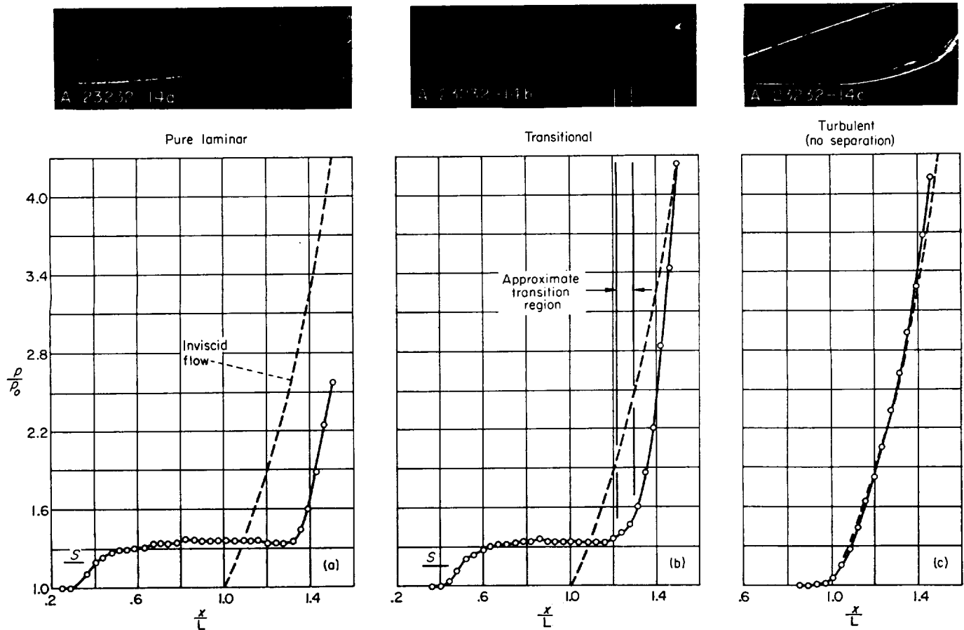
(a) CS25°-1; M_o=2.7 ; R_L=0.16 \times 10^6 . (b) CS25°-1 (trip 1); M_o=2.7 ; R_L=0.21 \times 10^6 . (c) CS25°-1 (trip 1); M_o=2.7 ; R_L=0.96 \times 10^6 .
