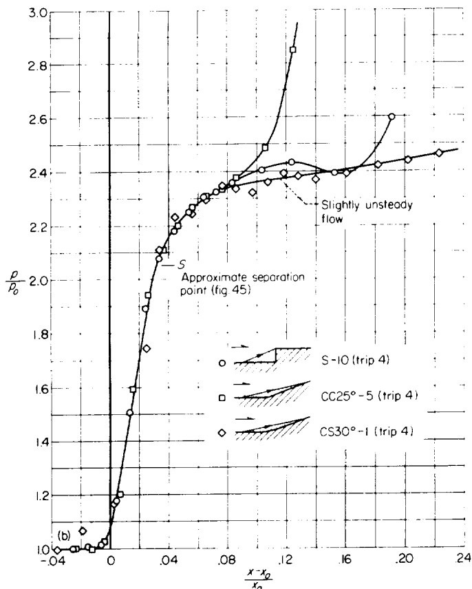
(b) M_0=3.0; R_{x_0}=3.1 \times 10^6
