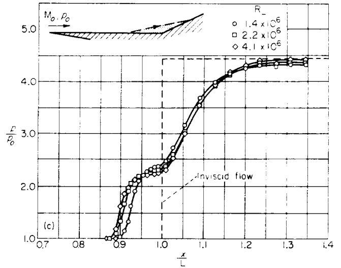
(c) Turbulent separation; CC25°-5 (trip 4); M_0=2.7 .
