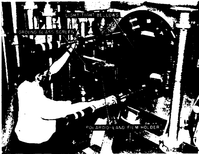
FIGURE 3.—Adjustable shadowgraph mount with light-tight bellows.
