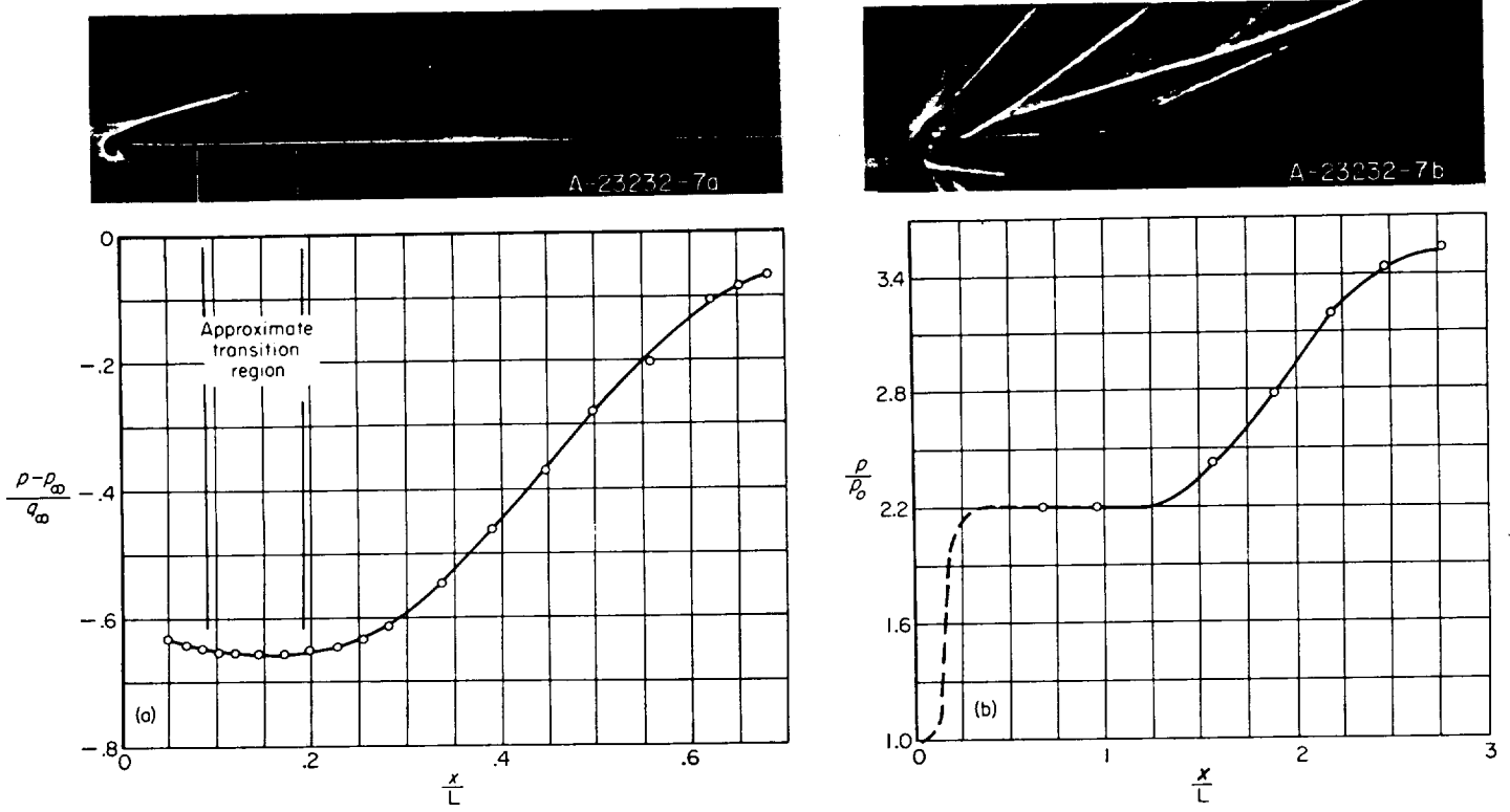
(a) Abrupt rise near reattachment of turbulent layer. S-9; M_\infty=0.47 ; \alpha=3^\circ ; R_L=0.68 \times 10^6 . (b) Abrupt rise near reattachment of thin laminar layer. CC20°-1; M_\infty=3.0 ; R_L=0.018 \times 10^6 FIGURE 10.—Examples of abrupt pressure rise not correlated with the location of transition.
