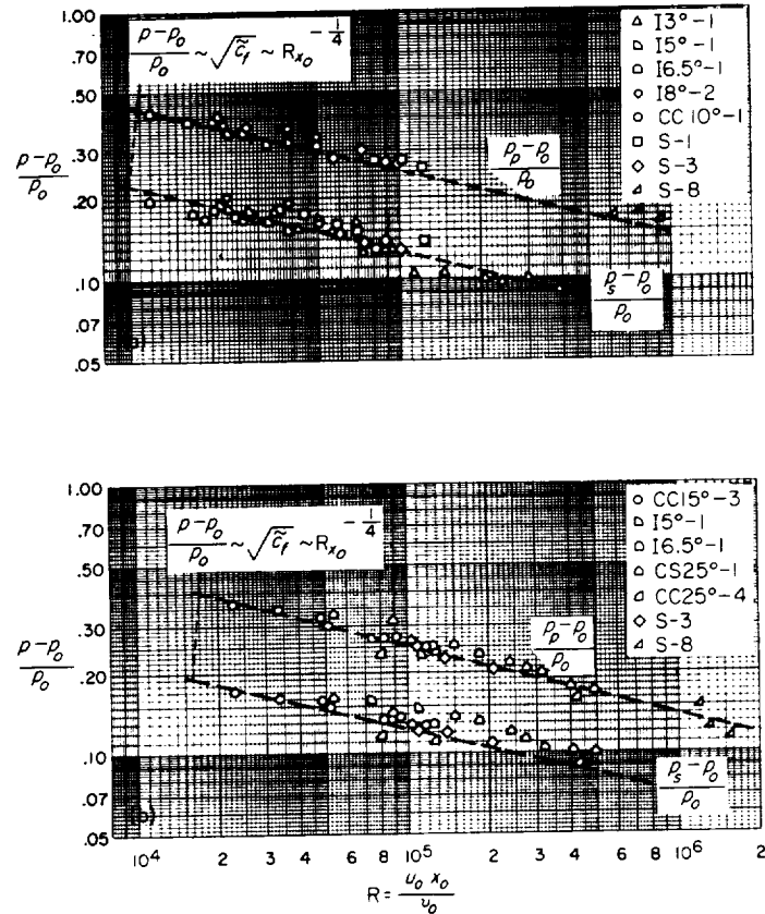
(a) Pure laminar separation; M_o=2.3 .
