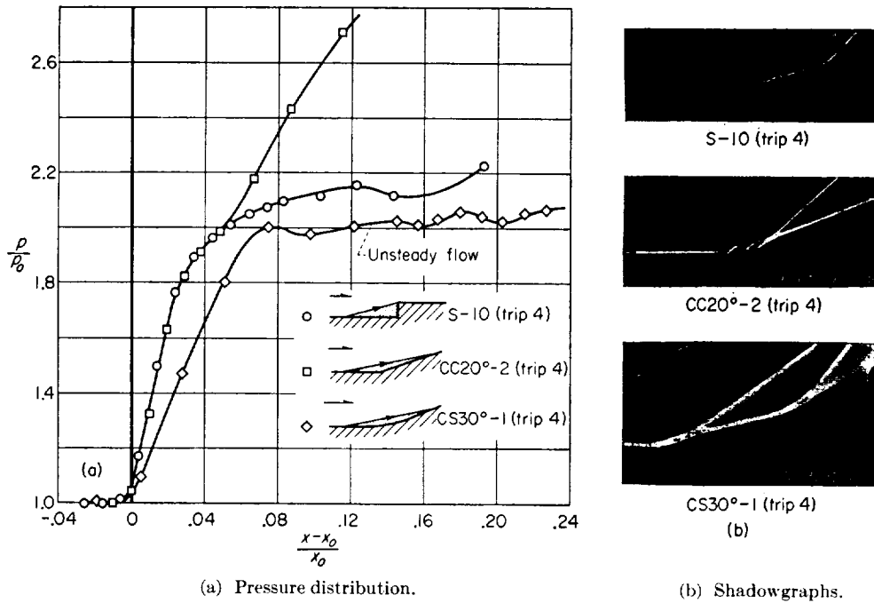
FIGURE 40.—Effects of flow unsteadiness on the pressure distribution and the corresponding shadowgraphs for turbulent separation; M_o=2.4 ; R_{x_0}=2.7 \times 10^6 .
