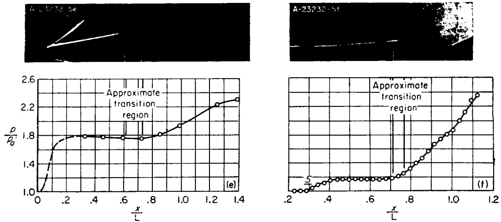
(e) CC15°-2; M_0=1.7 ; R_L=0.058 \times 10^6 . (f) CC25°-3; M_0=2.0 ; R_L=0.44 \times 10^6 .
