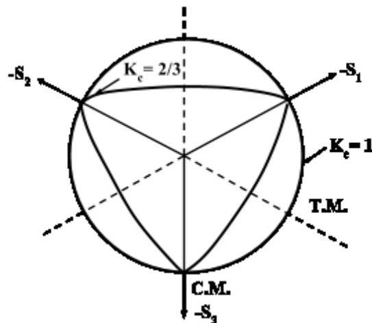
Figure 4 Yield surfaces in deviatory plane.
