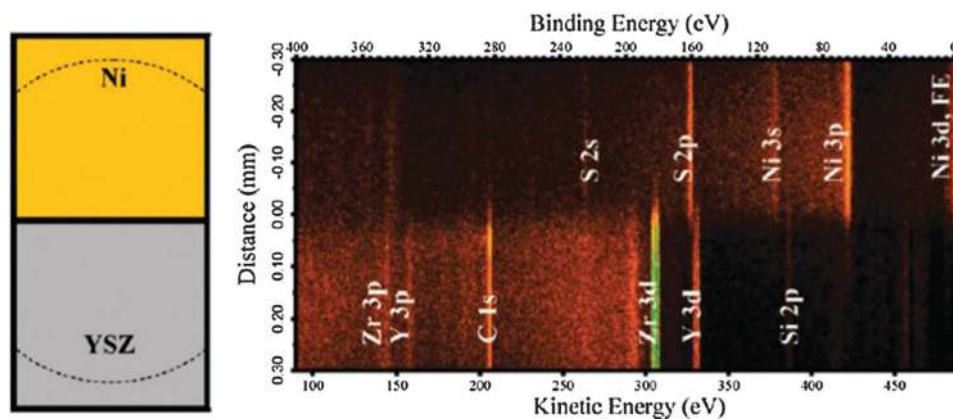
Fig. 11 Left panel: top-view schematic of the SOEC Ni/YSZ interface measured in the APXPS image (right). The dashed lines show the field-of-view (diameter \sim 0.6 mm). Right panel: the photoelectron binding energy versus real-space distance around the cell's three-phase boundary during operation at zero bias. Core level XPS peaks of Ni, YSZ, their impurities and the Ni Fermi edge (FE) are labeled. Intensities (counts) are displayed using a false-color scale. The binding energy scale is referenced to the Fermi edge of the grounded Ni electrode. Reproduced with permission from ref. 185.
