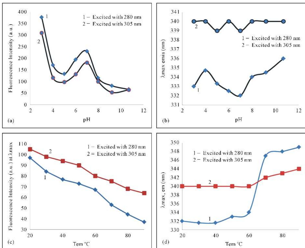
Figure 1. Comparative display of the change in fluorescence intensity and fluorescence wavelength of the surface and total tryptophan by selective excitation at 305 nm and 280 nm respectively at different pH ((a) and (b)) and temperature ((c) & (d)).
