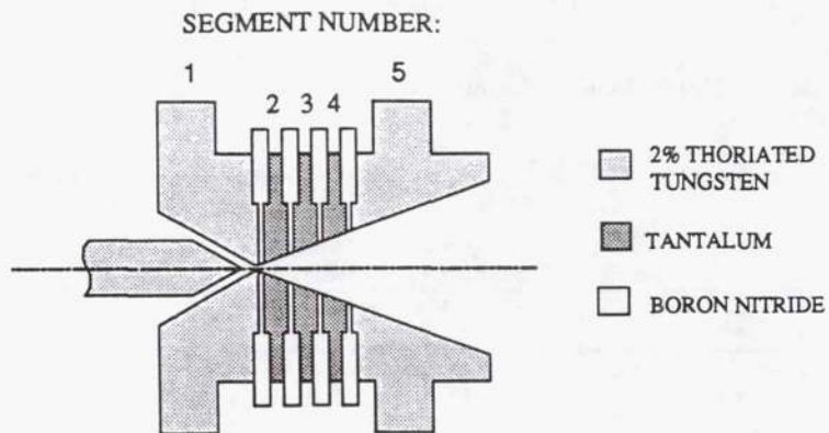
Figure 3. Thruster B anode/nozzle schematic
