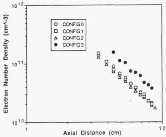
Figure 18. Electron number density as a function of axial distance on centerline at electrical configurations for Thruster B at 10A and a 1:2 N 2 /H 2 propellant flow rate of 49 mg/s.
