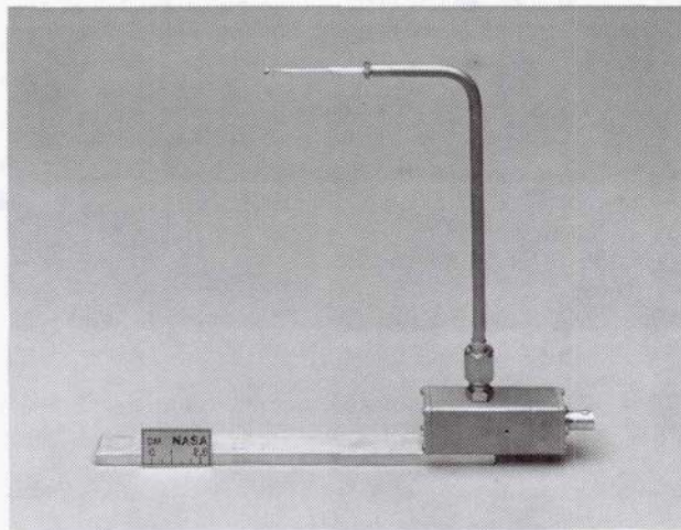
Figure 2. Spherical probe and probe support structure
