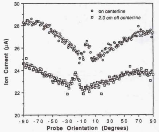
Figure 9. Ion current as a function of probe orientation at an axial distance of 8 cm. Arcjet Thruster A at 10A 115V with 1:2 N 2 /H 2 flow rate of 49 mg/s.
