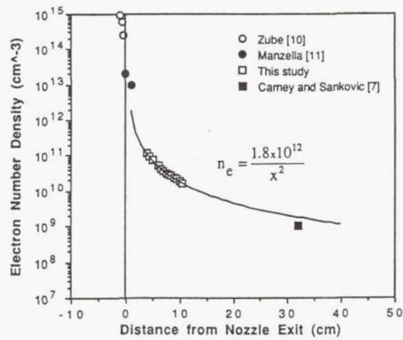
Figure 11. Electron number density at various axial distances on centerline. Comparison of data obtained in this study with previous data for other regions of the plume.
