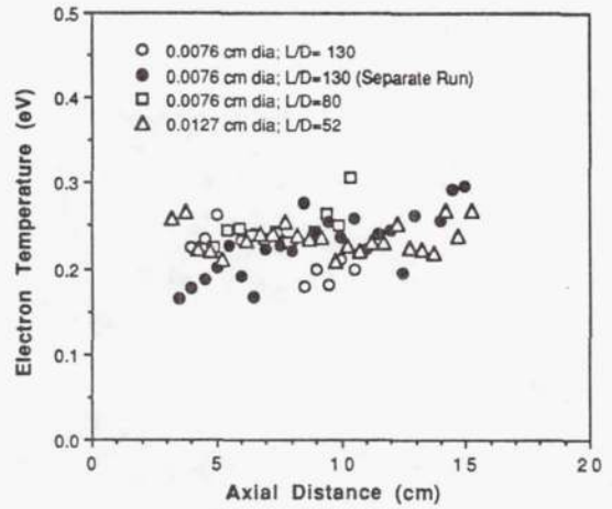
Figure 7. Electron temperature as a function of axial distance for various cylindrical probe geometries. Arcjet Thruster A at 10A 115V with 1:2 N 2 /H 2 flow rate of 49 mg/s.
