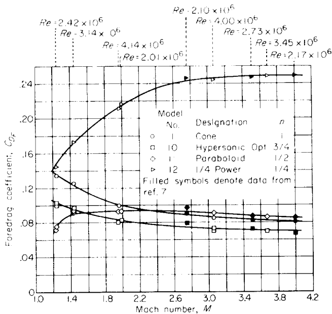
FIGURE 15.—Variation of foredrag coefficient with Mach number for the family of L/D=3 nose shapes defined by r=R\left(\frac{X}{L}\right)^n .
