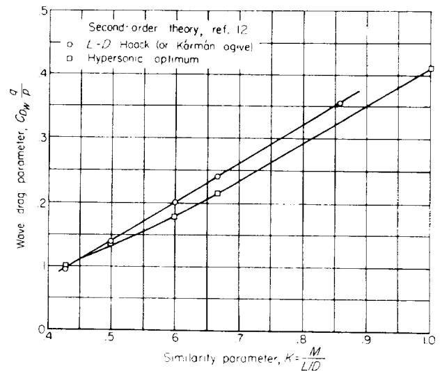
FIGURE 14.—Variation of wave drag parameter, (C_{Dw} q) / p , with the similarity parameter for the theoretical minimum drag nose shapes of specified length and diameter.
