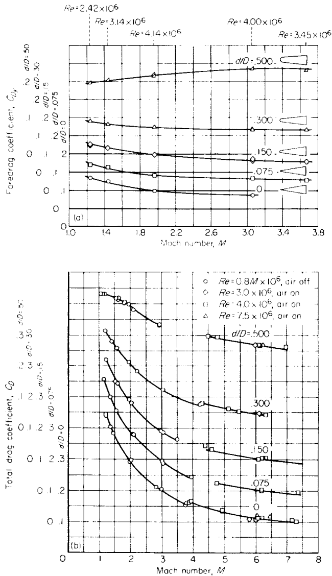
(a) Wind tunnel results. (b) Free-flight results. FIGURE 7.—Variation of drag coefficient with Mach number for hemisphere-cone series, constant \frac{L}{D}=3 .
