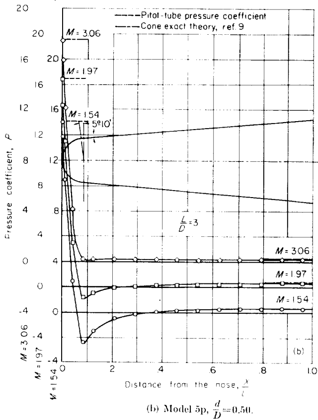
FIGURE 4.—Longitudinal distribution of pressure coefficient for hemisphere-cones at 0^\circ angle of attack.
