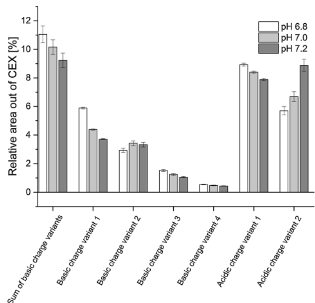
Fig. 4 Relative area out of cation exchange chromatography (CEX) for various charge variants and one sum parameter at different pH set points for p\text{CO}_2 12.5 % and p\text{O}_2 25 %
