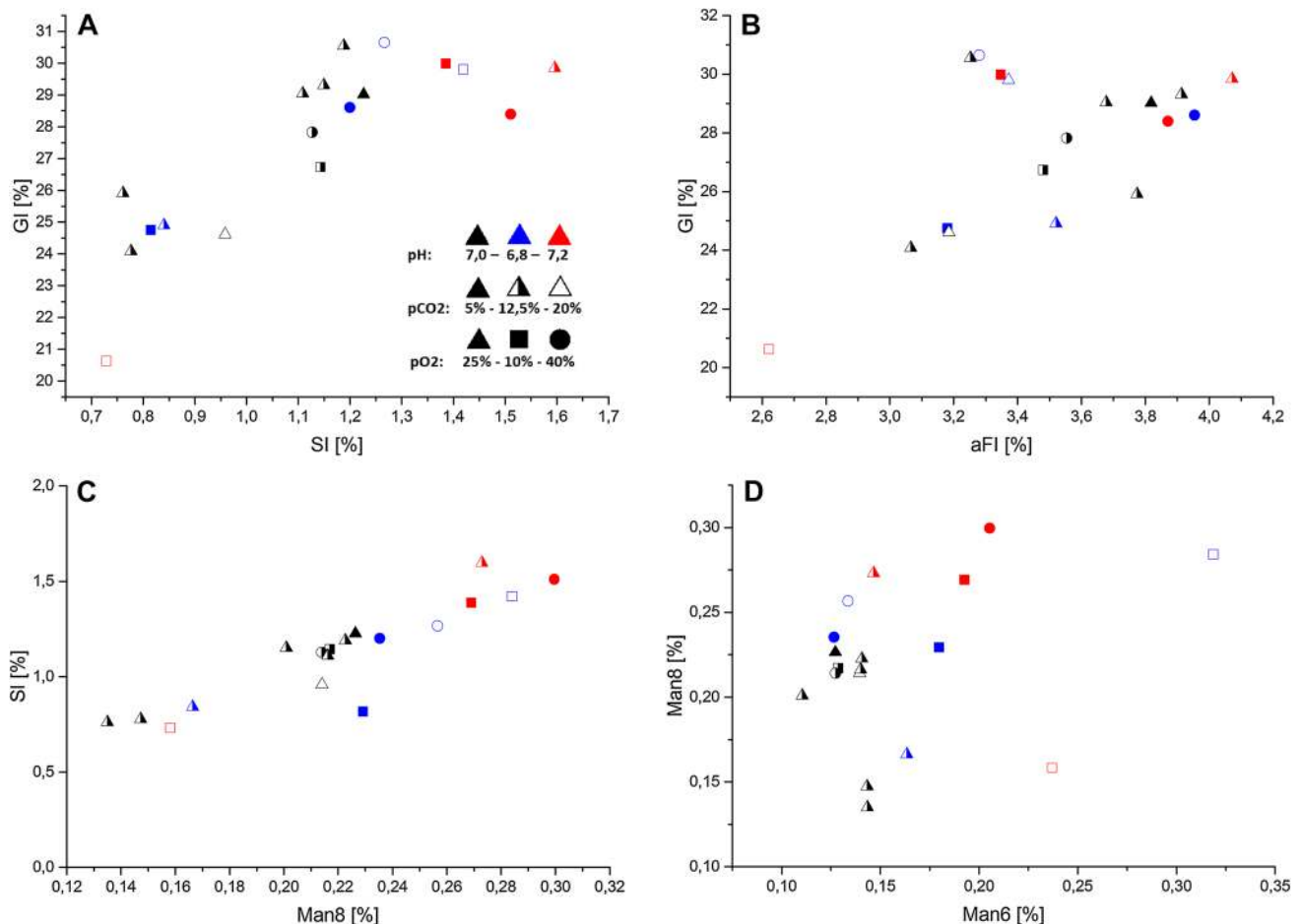
Fig. 5 Correlations and trends of glycosylation variants. (Black symbols represent processes at pH 7.0, blue symbols at pH 6.8, red symbols at pH 7.2; closed symbols represent processes at pCO 2 5%, half-closed at 12.5% and open symbols at 20%; triangles represent processes at pO 2 25%, squares at 10%, circles at 40%). Antibody galactosylation level (GI) over a sialylation (SI) and b afucosylation
