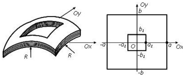
Fig. 1 A form of a shallow shell.
