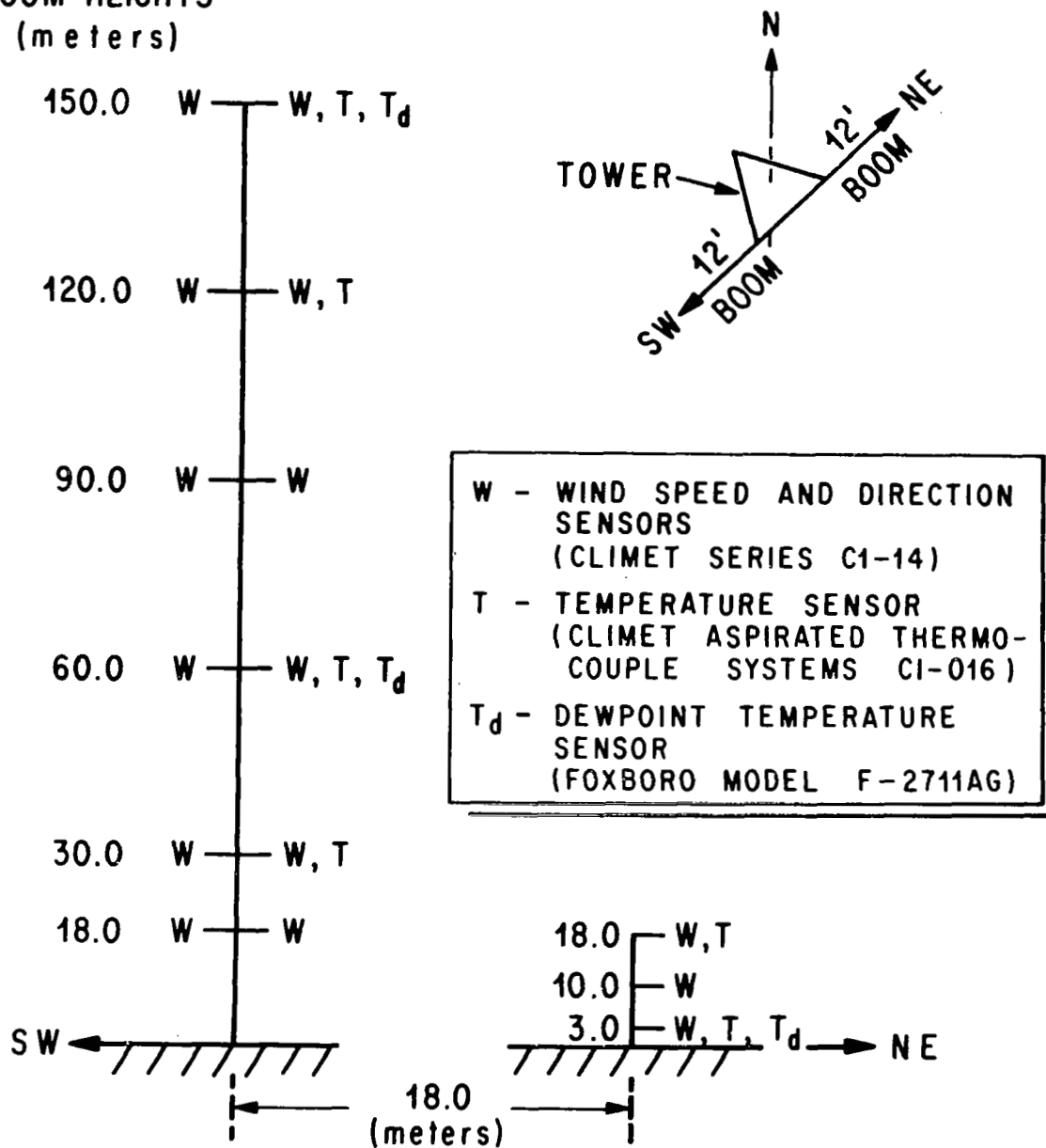
Figure 0.3 Schematic diagram of the NASA tower facility.
