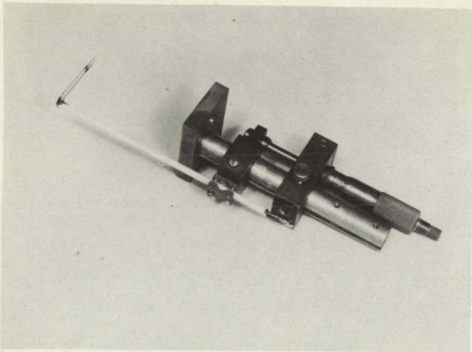
Figure 3.- Traversing mechanism.
