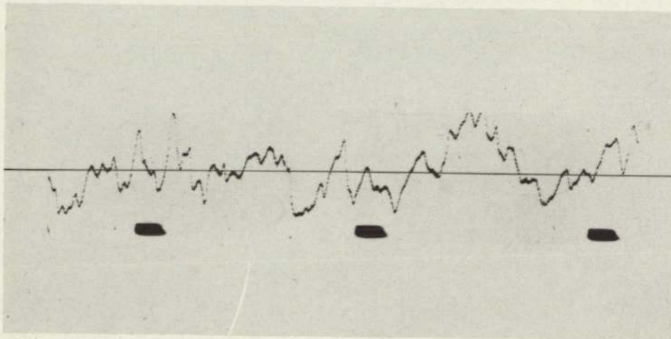
Figure 4.- Typical oscillogram of u' -fluctuation at R = 30,800 and y/d = 1.0 . Horizontal line corresponds to u'(t) = 0 ; interval is approximately 1/20 second.
