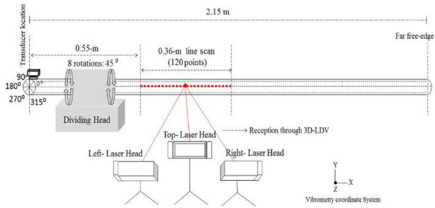
Fig. 10. 3D-LDV setup.
