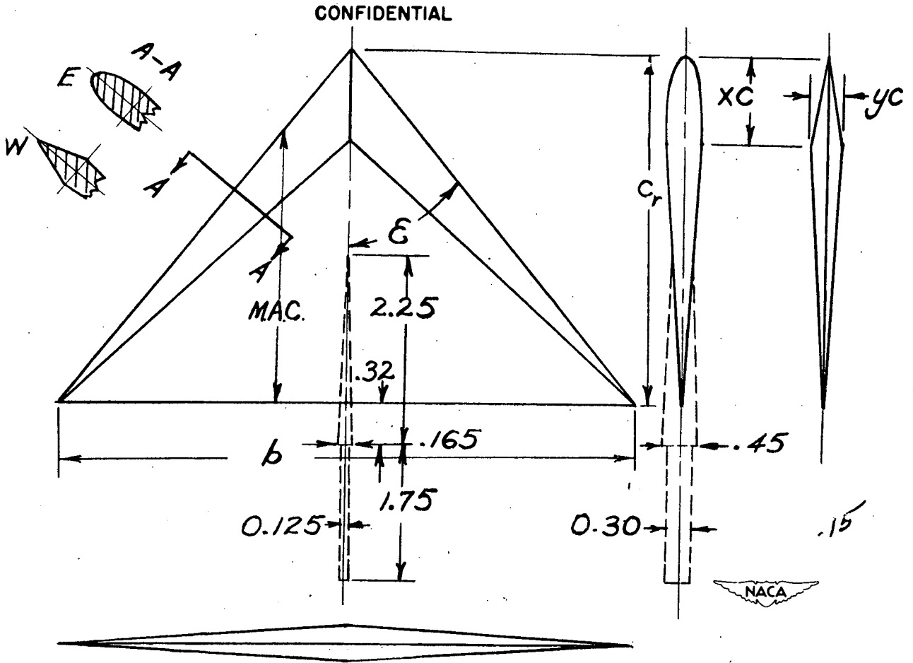
Figure 2.— Dimensions of 8-percent-thick triangular-wing models. (Sting dimensions identical for all wings. E, elliptical leading edge; W, wedge leading edge.) CONFIDENTIAL
