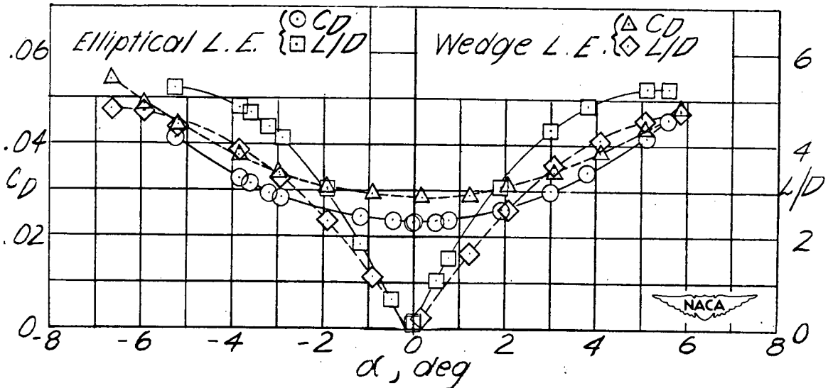
(e) Wing 5. w=0.675 ; R=1,080,000 .
