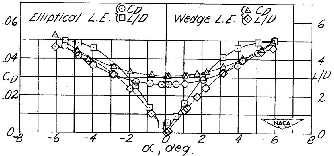
(f) Wing b/w = 0.731 ; R = 1,000,000 .
