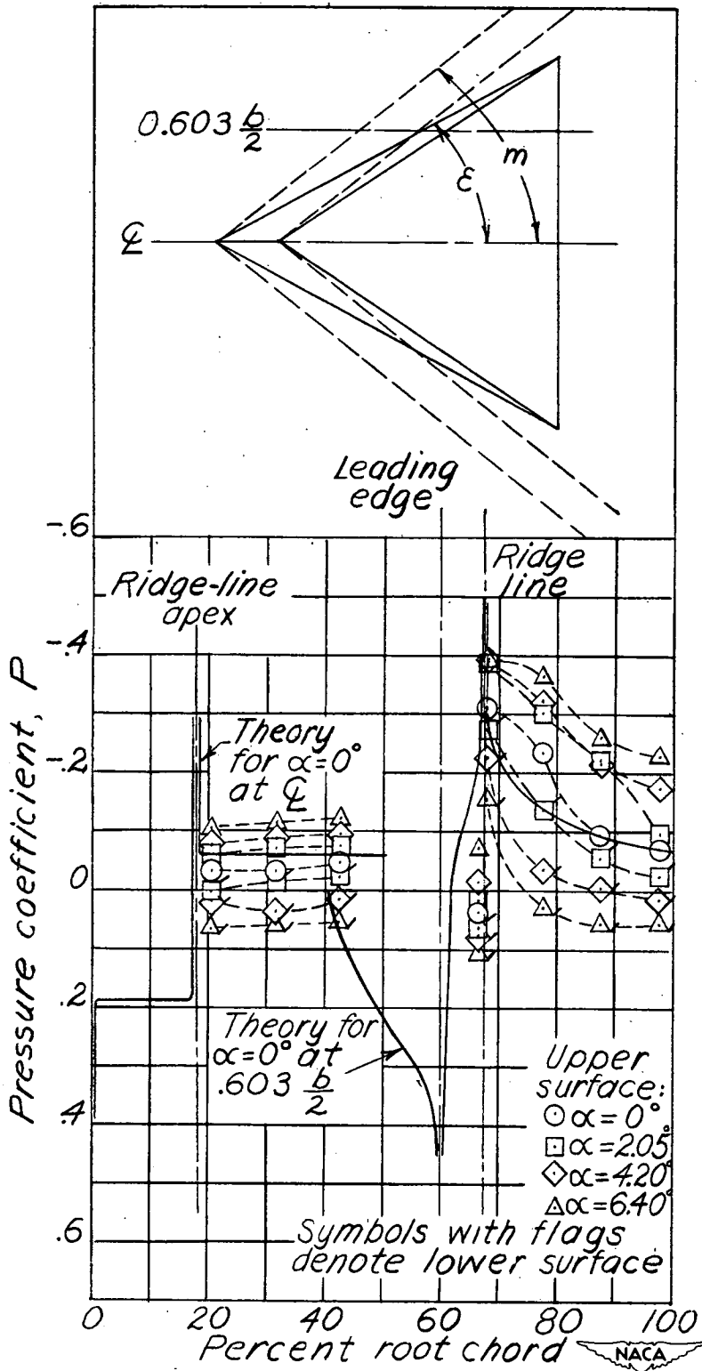
(b) 60.3 percent semispan and root station, \zeta Figure 21. - Concluded.
