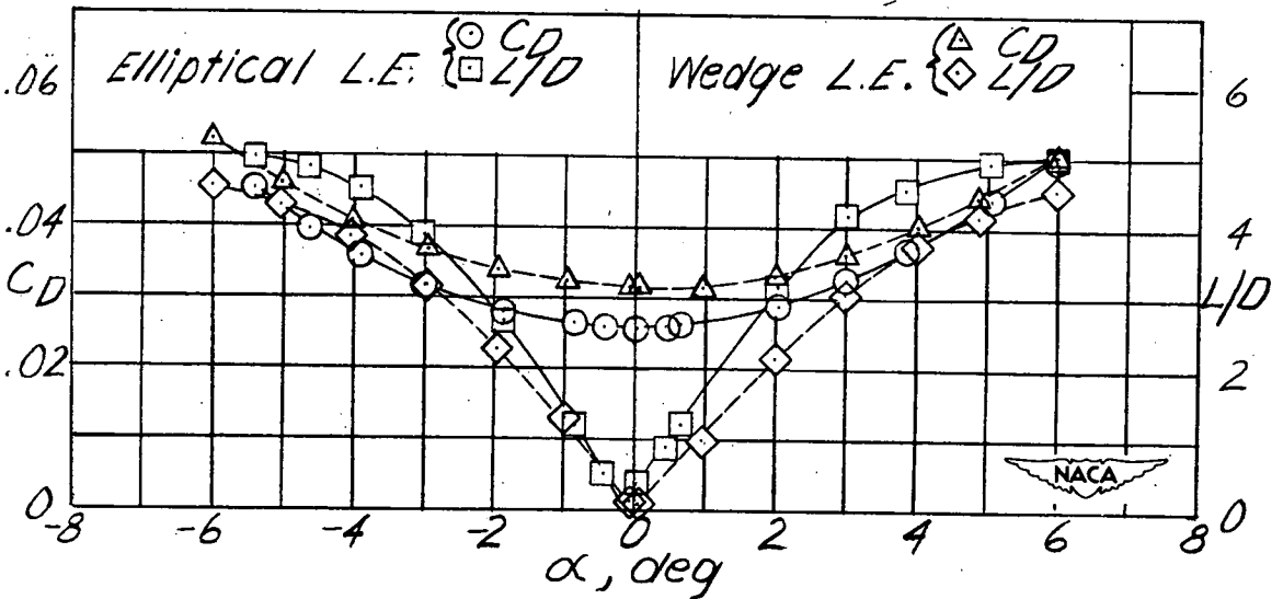
(g) Wing 7.w=0.801 ; R = 940,000 .
