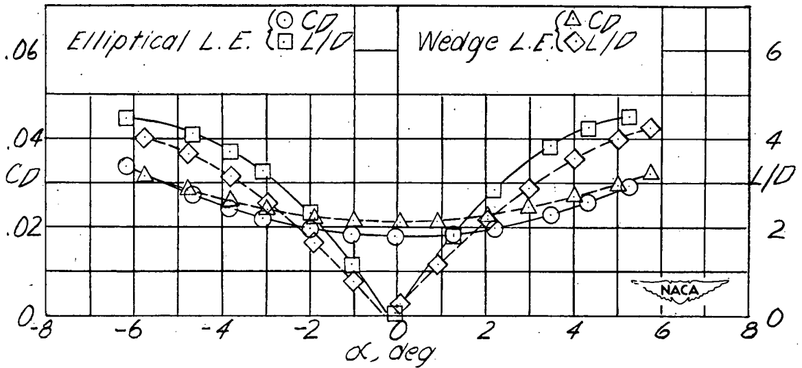
(c) Wing 3. w = 0.880 ; R = 990,000 .
