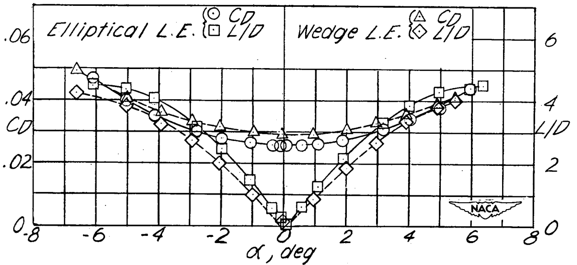
(f) Wing 6. w=0.940 ; R = 900,000 .
