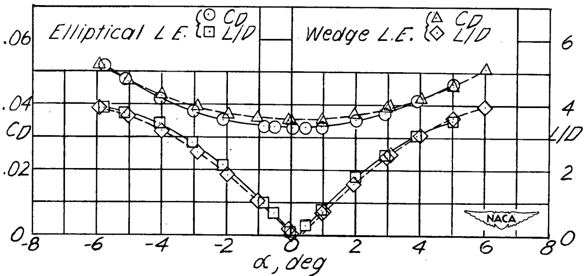
(j) Wing 10. w=1.371 ; R=660,000 .
