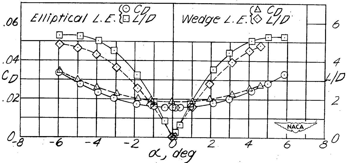
(b) Wing 2. w=0.530 ; R=1,250,000 .
