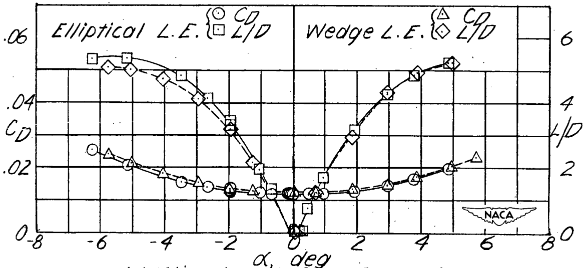
(a) Wing 1. w=0.287 . R=1,250,000 . Figure 6. -Aerodynamic characteristics of .8-percent-thick triangular wings at M=1.92 .
