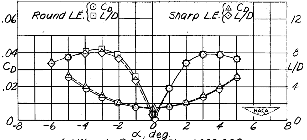
(a) Wing 1. R (round LE) = 1,060,000. Figure 8.- Aerodynamic characteristics of flat-plate triangular wings at M = 1.92 .
