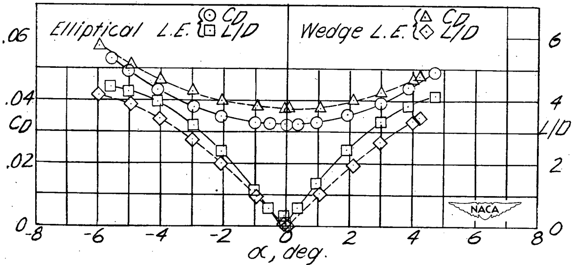
(i) Wing 9. w = 0.996 ; R = 780,000 .
