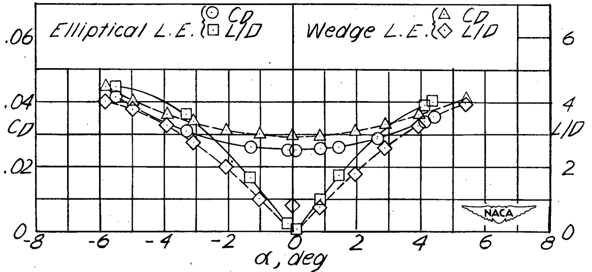
(g) Wing 7. w=1.030 ; R = 840,000 .
