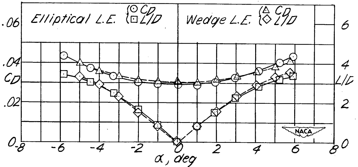
(h) Wing 8. w=1.540 ; R = 620,000 .
