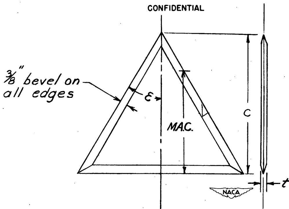
Figure 3.— Dimensions of flat-plate triangular-wing models. (Sting supports identical with thick-wing installation.)
