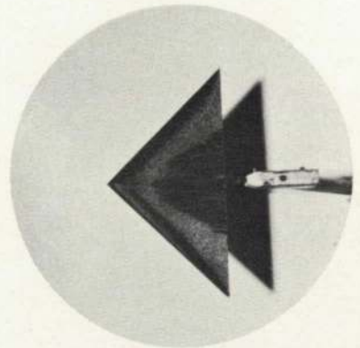
(b) Elliptical-leading-edge wing ll. \alpha = 4^\circ , upper surface.
