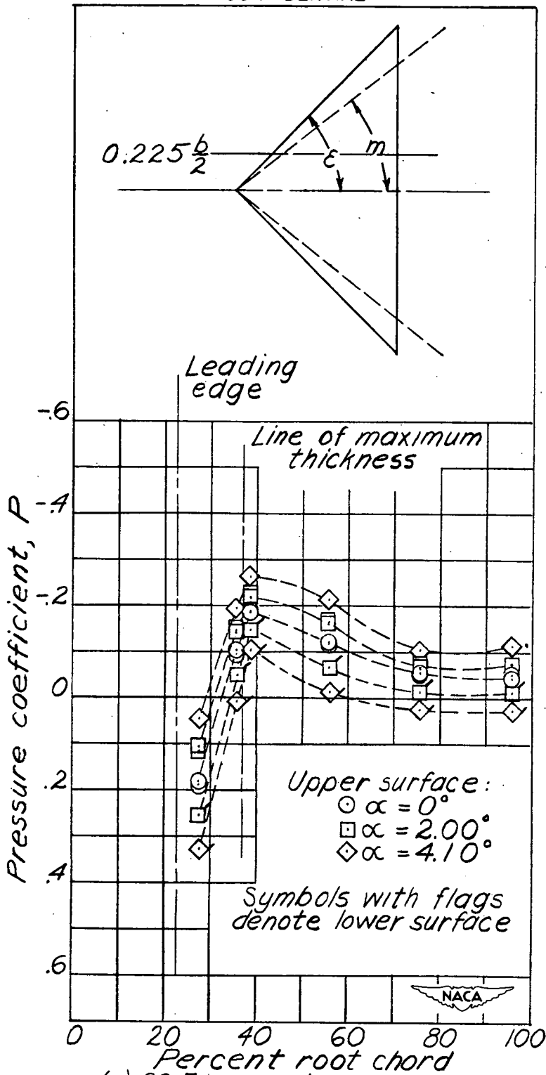
(a) 22.5 percent semispan. Figure 23.—Pressure distribution at varying angle of attack on elliptical-L.E. wing II at M=1.62 . \tan \epsilon / \tan m > 1 .
