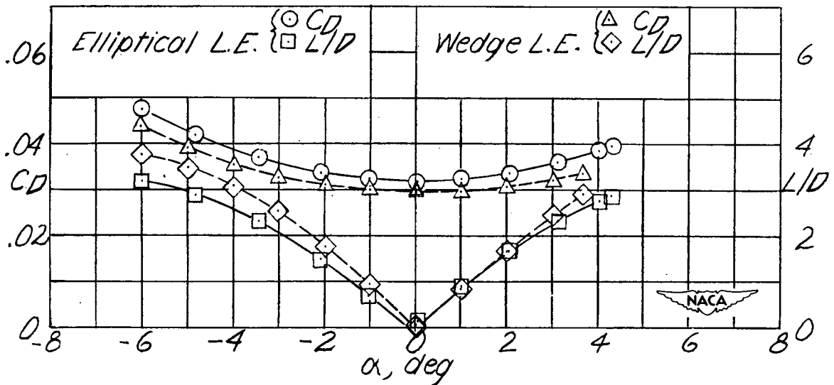
(i) Wing 9. w = 1.705 ; R = 560,000 .
