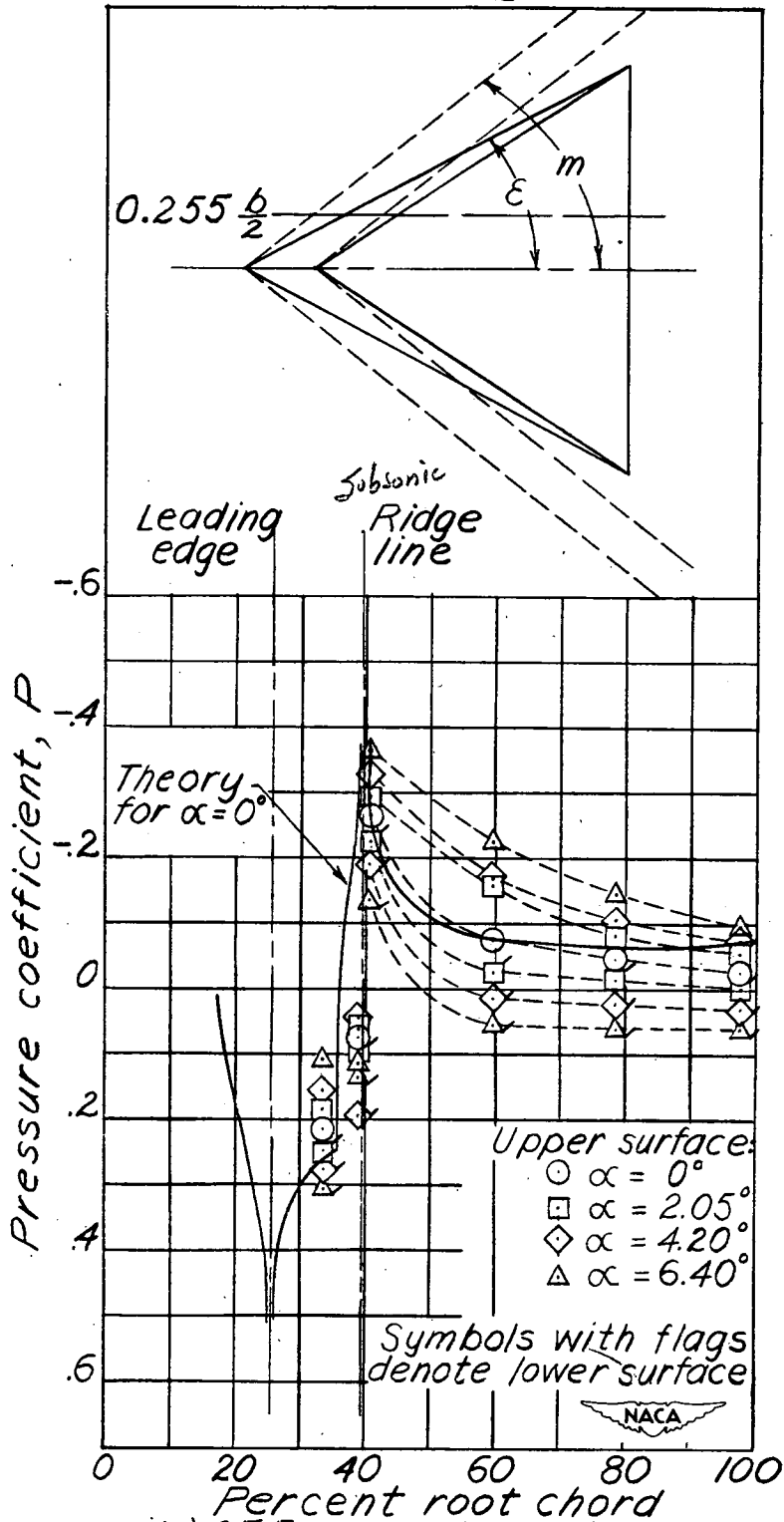
(a) 25.5 percent semispan.
