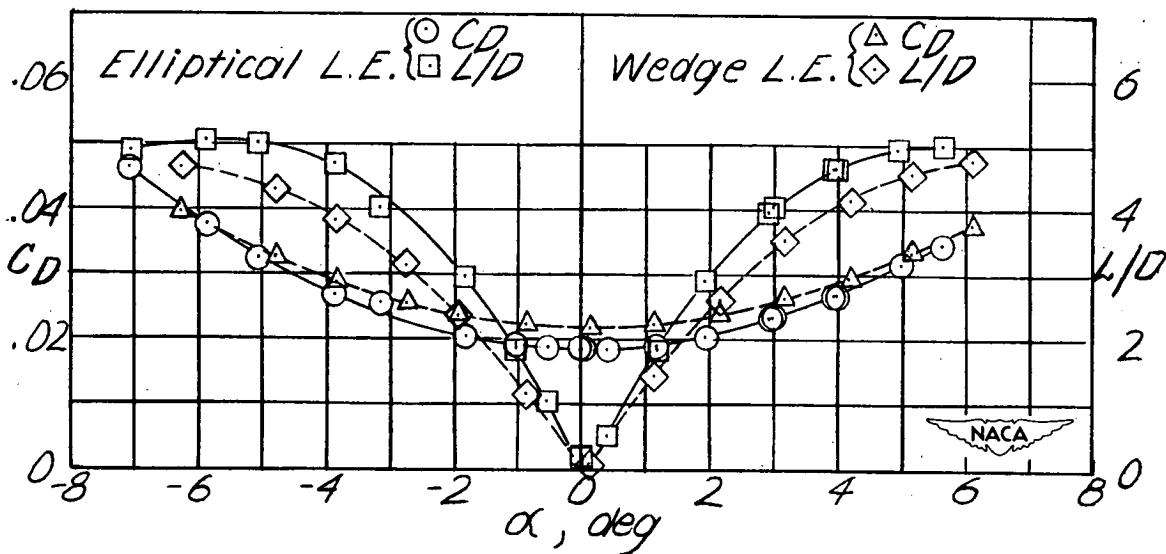
(c) Wing 3. w=0.661 ; R=1,230,000 .
