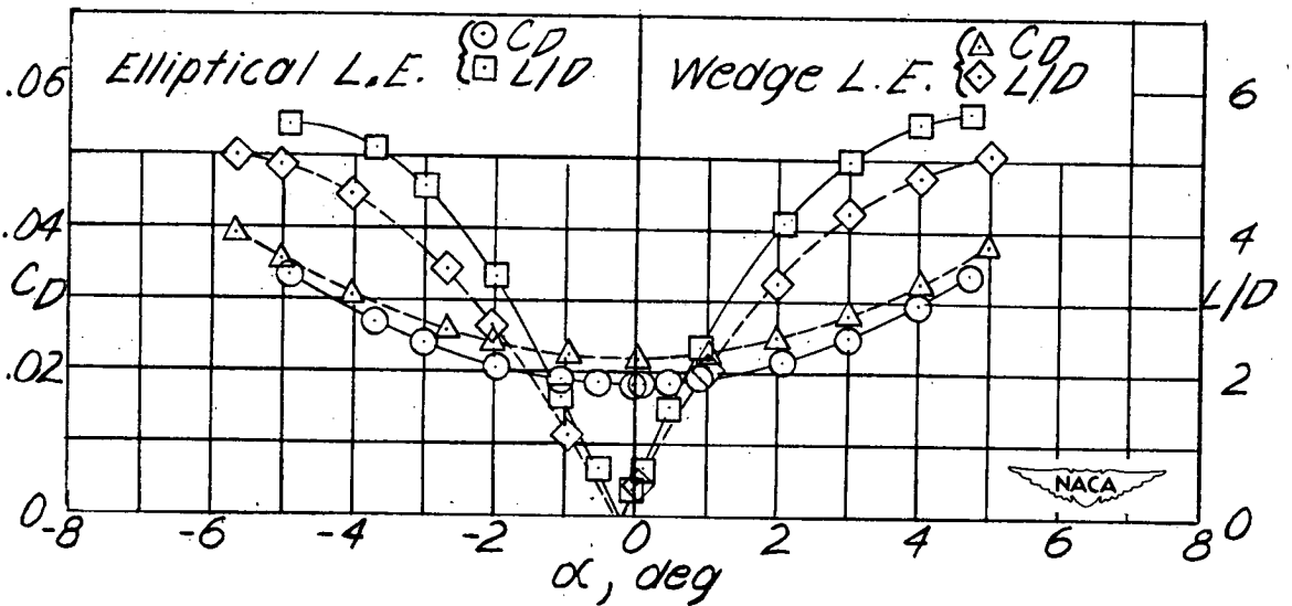
(c) Wing 3. w=0.514 ; R=1,380,000 .
