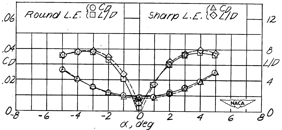
(b) Wing 2. R (round L.E.) = 850,000.
