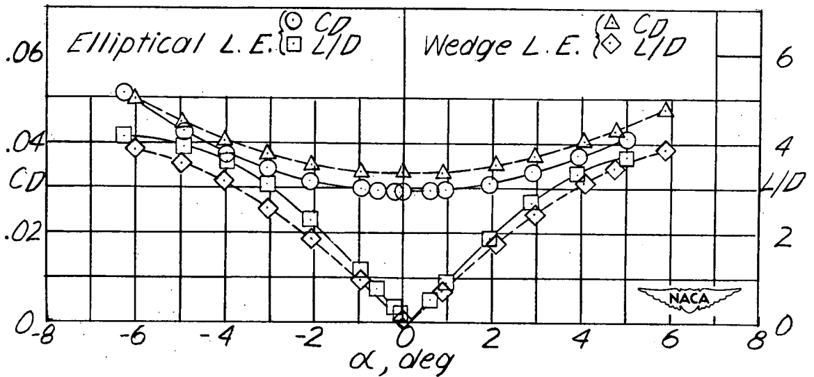
(h) Wing 8.w=1.156 ; R = 770,000 .
