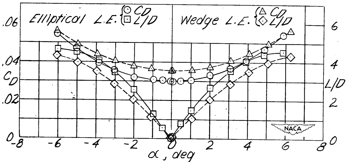
(h) Wing B.w = 0.899 ; R = 860,000 .
