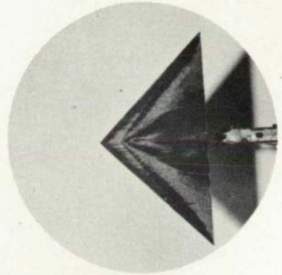
(a) Wedge-leading-edge wing ll. \alpha = 4^\circ , upper surface.
