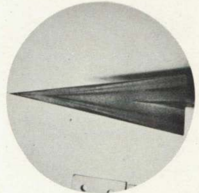
(c) Wedge-leading-edge wing l. \alpha = 4^\circ , upper surface.
