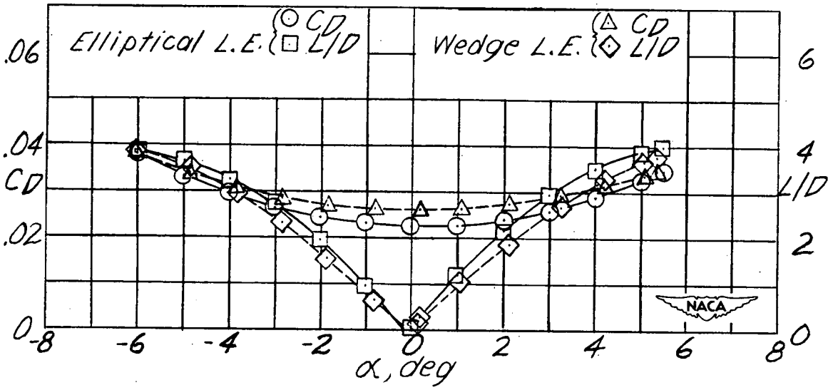
(e) Wing 5. w=1.156 ; R = 770,000 .
