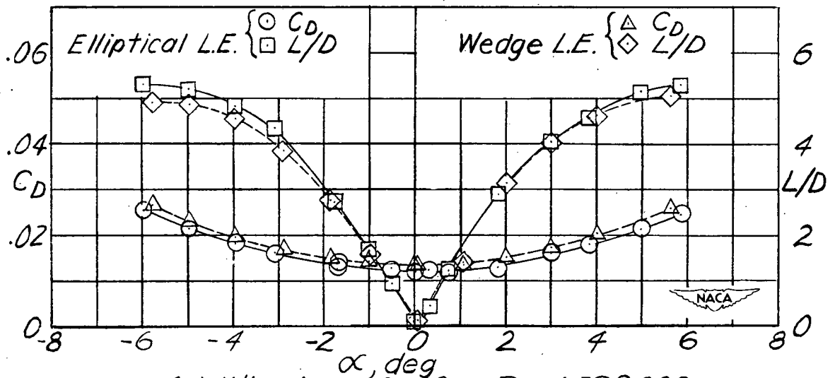
(a) Wing 1. w=0.223 . R=1,390,000 . Figure 5.- Aerodynamic characteristics of 8-percent-thick triangular wings at M=1.62 .
