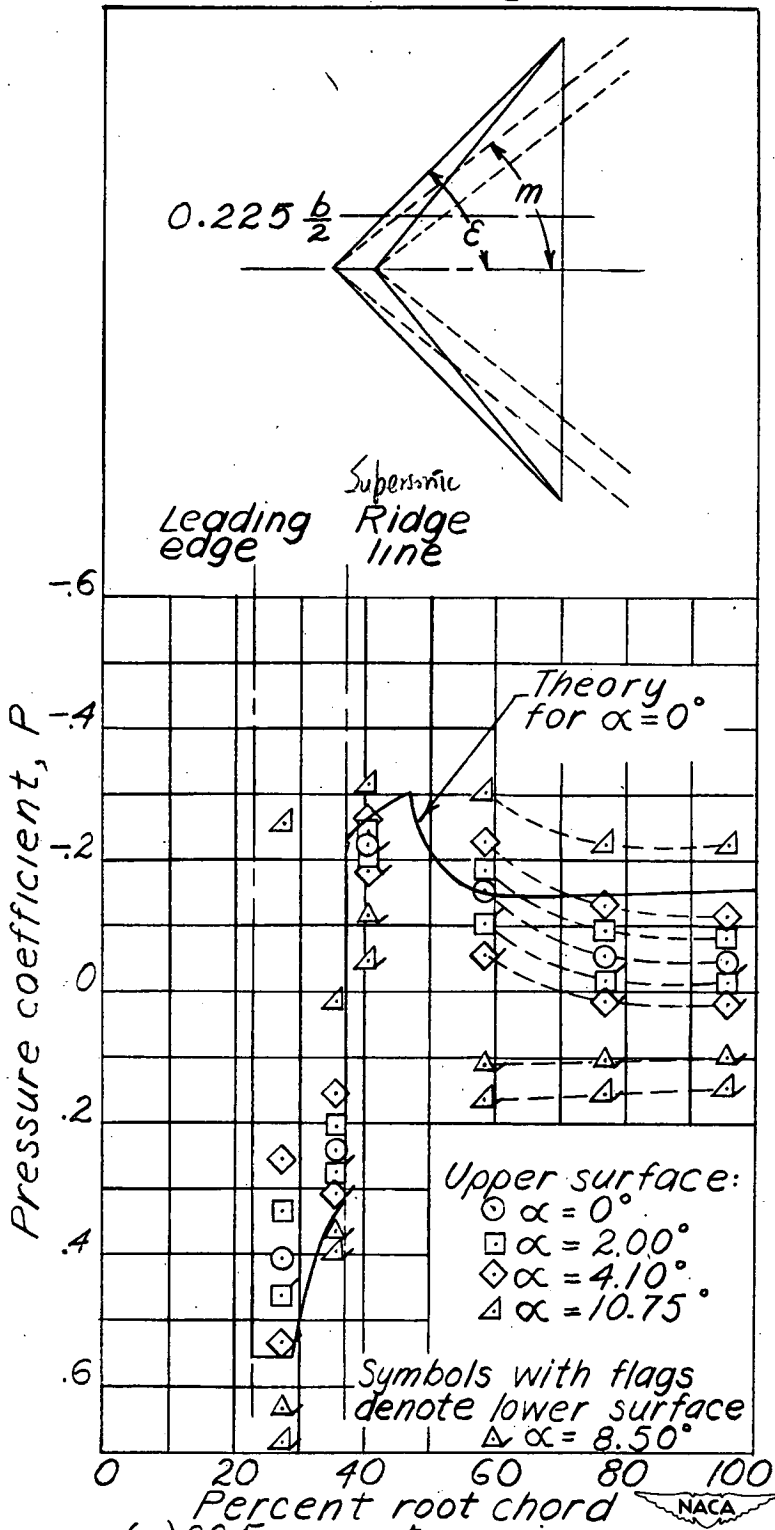
(a) 22.5 percent semispan.
