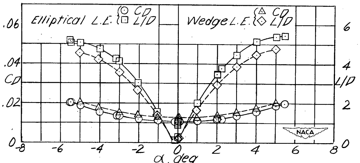
(a) Wing I. w = 0.382 ; R = 1,000,000 . Figure 7. - Aerodynamic characteristics of 8-percent-thick triangular wings at M = 2.40 .
