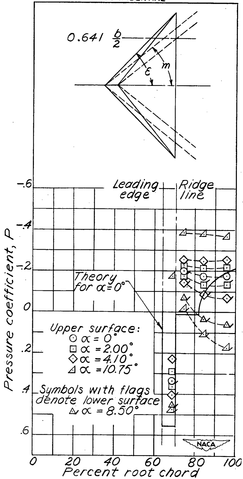
(b) 64.1 percent semispan. Figure 22.- Concluded.
