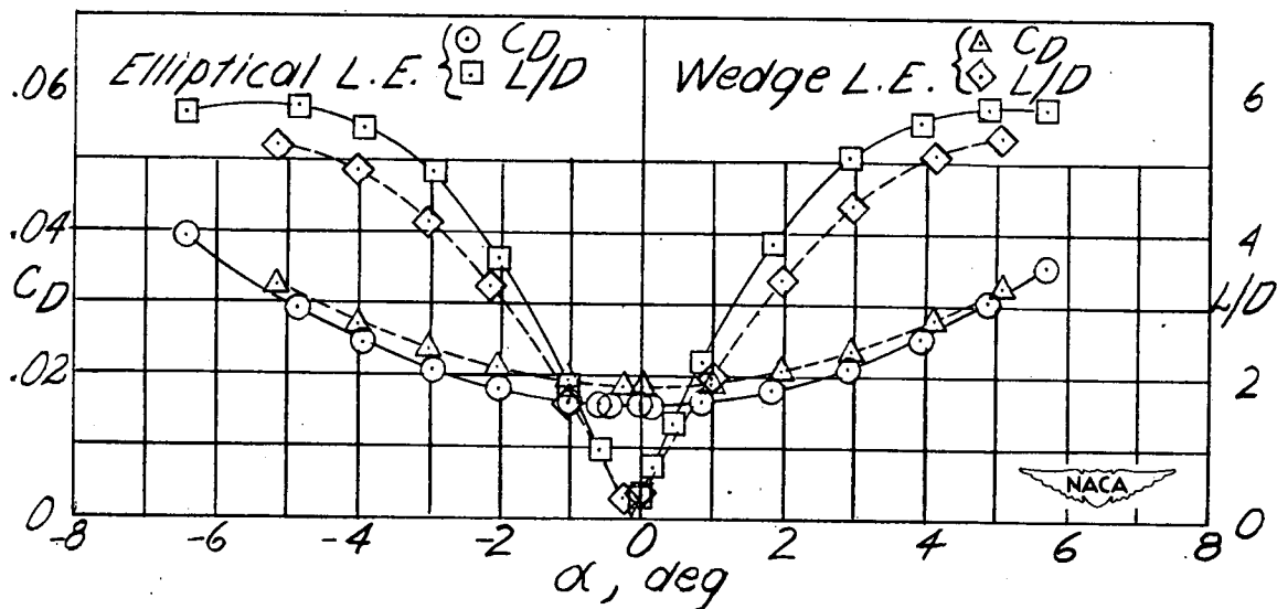
(b) Wing 2. w = 0.412 ; R = 1,390,000 .
