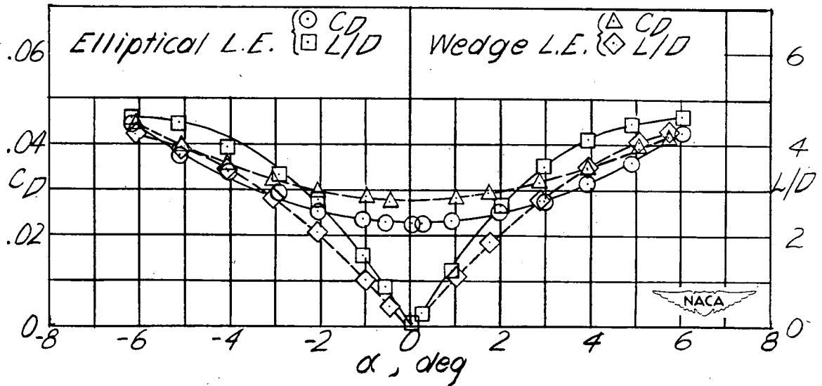
(e) Wing 5. w=0.869 ; R = 960,000 .
