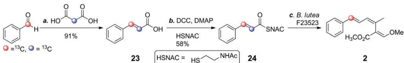
Scheme 2 Reagents and conditions: (a) [2\text{-}^{13}\text{C}] -malonic acid (1.02 equiv.), \text{Na}_2\text{SO}_4 (0.15 equiv.), pyridine, piperidine, reflux, 4 h, 91%; (b) DCC (1.13 equiv.), DMAP (0.04 equiv.), HSNAC (1.43 equiv.), DCM, 0 ^\circ\text{C} , 2 h, 23 ^\circ\text{C} , 16 h, 58%.
