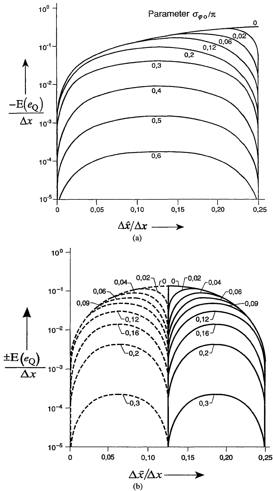
FIGURE 1 (a) Expected value of the quantization error as a function of the residual section \Delta \hat{x} of the deflection amplitude \hat{x} . \Delta \hat{x} defined by Eq. (12), zero-phase angle \varphi_0 is narrow band stochastic process of 2nd order with: resonance rise Q = 10 , expected value E(\varphi_0) = 0 + \mu\pi , \mu = 0, \pm 1, \pm 2, \dots , standard deviation \sigma_{\varphi_0} . (b) The same but with expected value E(\varphi_0) = \pi/4 + \mu\pi .
