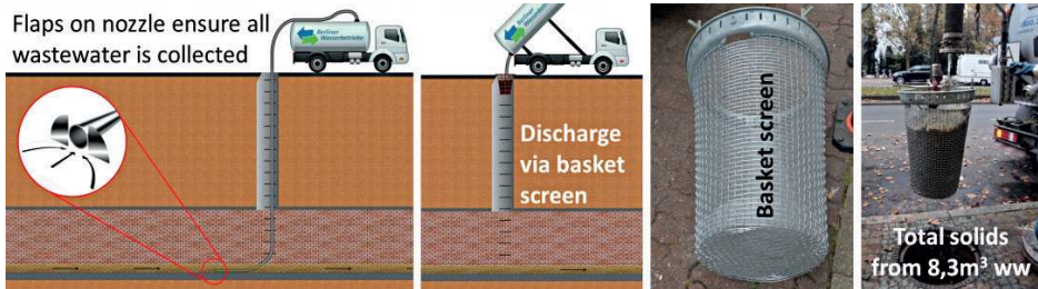
Fig. 5. From left to right: Wastewater being collected with the suction vehicle, wastewater being discharged into the sewers through the basket screen, basket screen, basket screen with solids captured from 8.3 m 3 of wastewater
