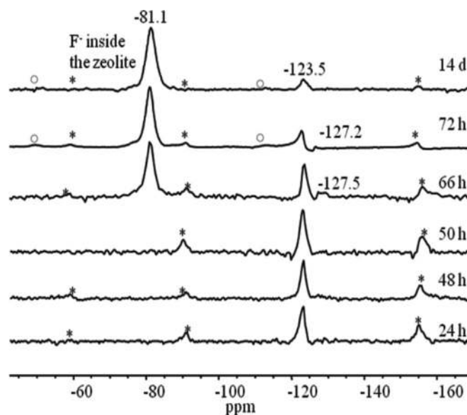
Fig. 5. ^{19}\text{F} MAS NMR spectra of samples obtained from the reactions quenched at different time intervals. A spinning speed of 12 kHz was used. The spinning sidebands are shown by "*" and "o".
