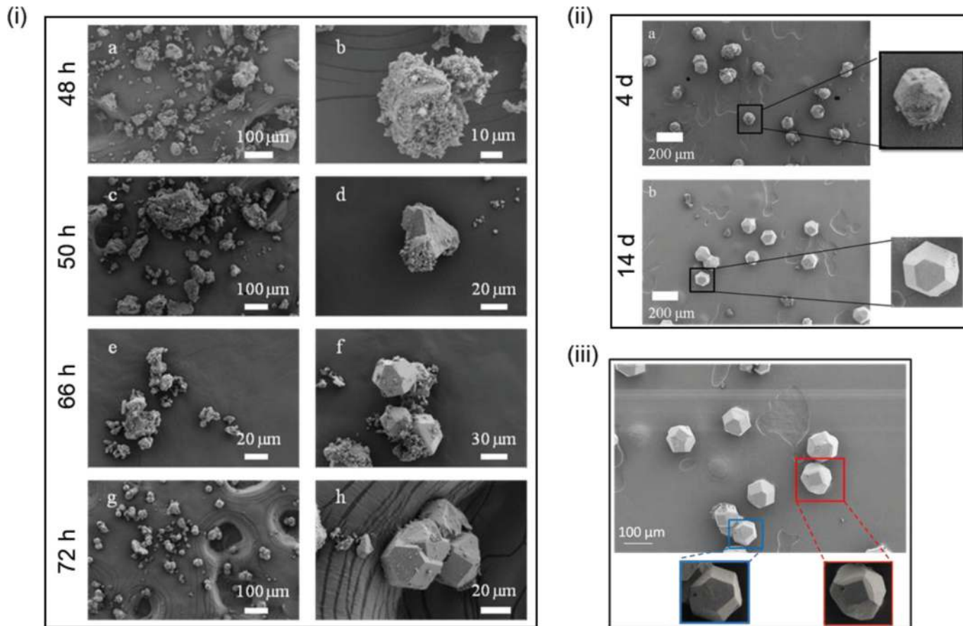
Fig. 6. (i) SEM images of samples obtained from the reactions quenched at 48 h (a and b), 50 h (c and d), 66 h (e and f), and 72 h (g and h). (ii) SEM images of the samples obtained from the reactions quenched at (a) 4, and (b) 14 days. (iii) SEM image of ZSM-39 crystals and two magnified images shown (100) and (111) faces. [Colour online.]
