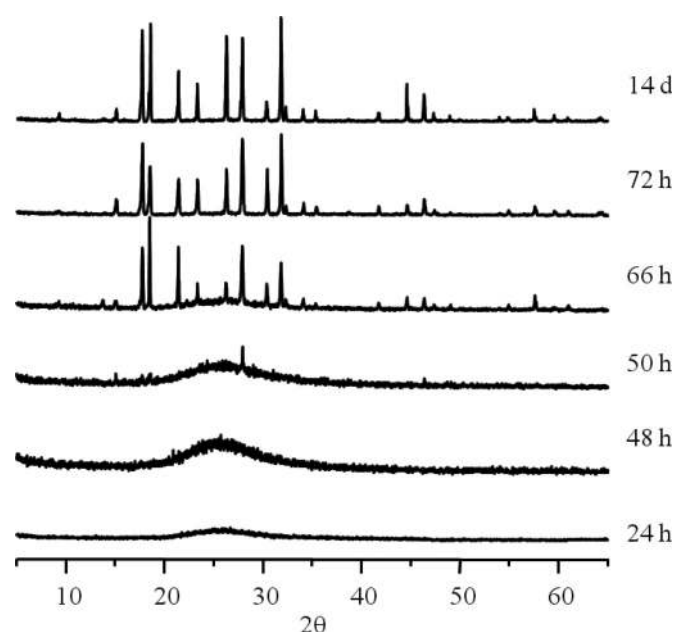
Fig. 2. PXRD patterns of the samples obtained by quenching the reactions at different time intervals.
