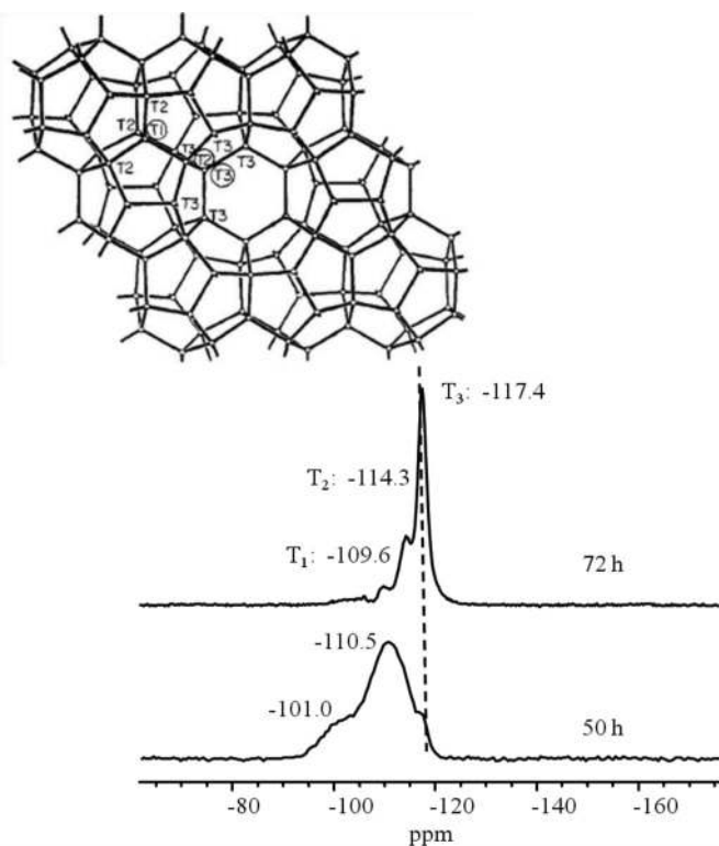
Fig. 7. ^1\text{H} \rightarrow ^{29}\text{Si} CP MAS NMR spectra of the 50 h sample (contact time = 10 ms) and a 72 h sample (for comparison). The framework structure of ZSM-39 with labeled T-sites are shown. 32
