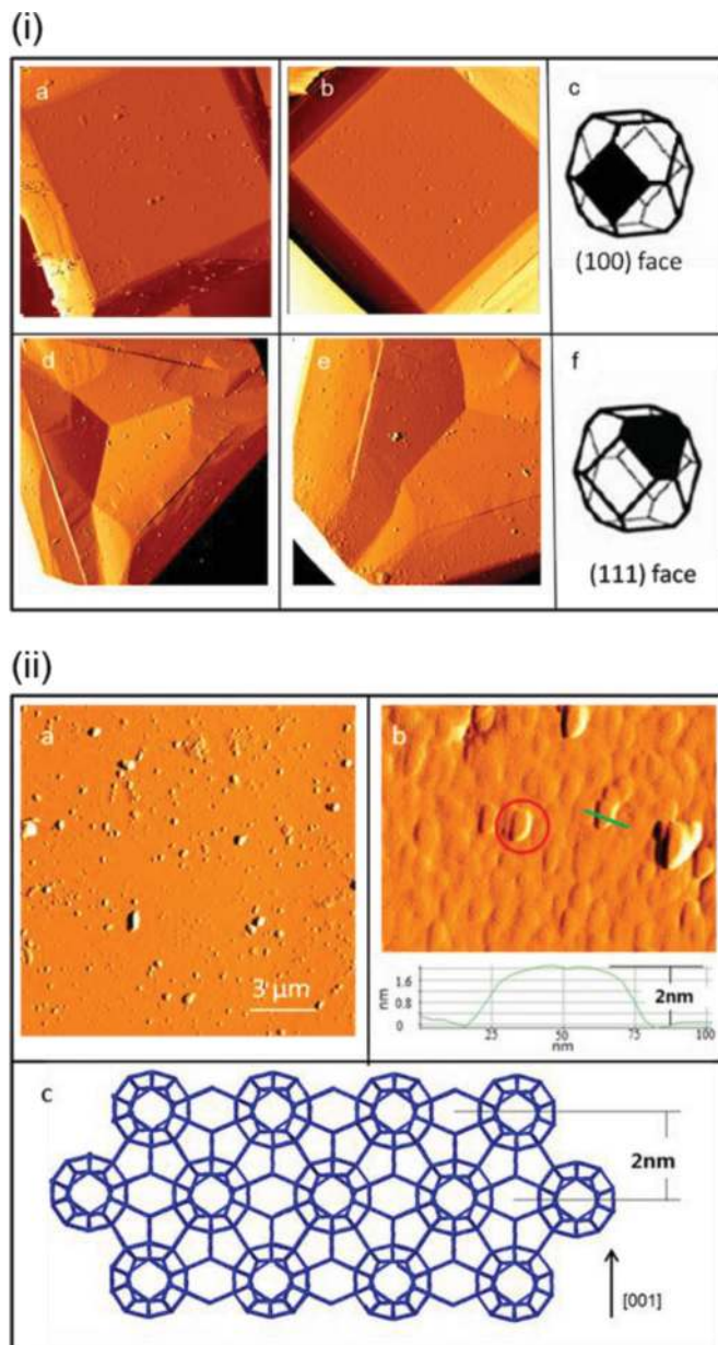
Fig. 8. (i) AFM error signal images (scan area: 45\ \mu\text{m} \times 45\ \mu\text{m} ) of ZSM-39: (a and b) overview images on (100) faces, (d and e) overview images on (111) faces. (ii, a) AFM error signal image on the (100) face of ZSM-39; (ii, b) magnified image on a flat area and a cross-section profile obtained from its corresponding topographic image (not shown); (ii, c) illustrative scheme of growth on along \langle 100 \rangle direction. [Colour online.]
