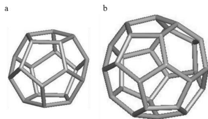
Fig. 1. Two types of cages that MTN structure is built upon: (a) [5^{12}] and (b) [5^{12}6^4] .
