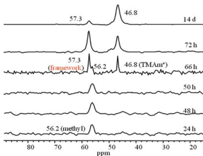
Fig. 4. ^1\text{H} \rightarrow ^{13}\text{C} CP MAS NMR spectra of samples obtained from reactions quenched at different time intervals. \text{TMAm}^+ = trimethylammonium ion. [Colour online.]
