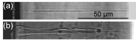
FIG. 2. Typical example of damage tracks in borosilicate glass (Corning 0211, a material close to BK7) after illumination with Bessel beams. The 800 nm laser pulses have an energy of 14.6 \mu\text{J} . The Bessel cone angle in the material is \theta = 10^\circ . The pulse durations are (a) 135 fs and (b) 3 ps.
