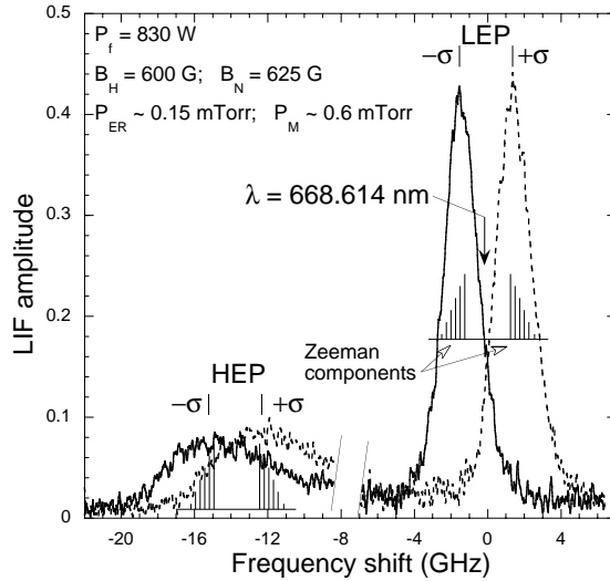
Figure 2: Laser-induced fluorescence amplitude vs. frequency shift at z = 1 cm in the ER. 0 GHz corresponds to the unshifted quartet 3d^4F_{7/2} - 4p^4D_{5/2} wavelength. The Zeeman effect splits the quartet into + and - \sigma components. Peaks near 0 GHz are termed the Low Energy Peaks (LEP). Peaks with frequency shifts greater than \sim 6 GHz are termed High Energy Peaks (HEP).
