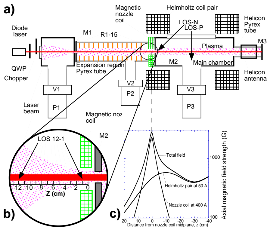
Figure 1: Schematic of the Magnetic Nozzle Experiment (MNX). a) Argon plasma is formed by absorption of helicon waves launched from a double-saddle antenna. The plasma flows through the main chamber along magnetic field lines created by a set of Helmholtz coils. The plasma then flows through metal aperture M2 and the nozzle coil into the expansion region (ER). The beam of a diode laser is directed along the MNX axis, allowing LIF measurements throughout MNX. b) Scanning mechanism for the LIF collection optics allows 12 lines-of-sight (LOS) intercepting axial points in the ER near the nozzle. c) Axial magnetic field strength near the nozzle coil.
