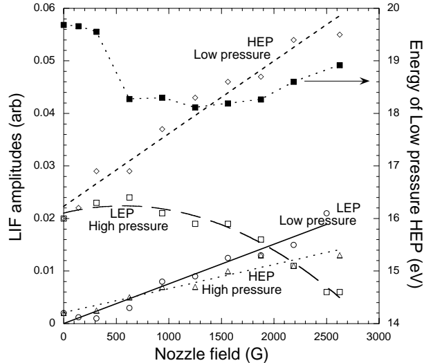
Figure 5: Effect of nozzle magnetic field strength on the LEP and HEP amplitudes for two ER pressures. The energy of the HEP at low p_{ER} is also shown. The absolute value of energy is uncertain to \pm 2 eV; the relative value to \pm 0.4 eV. The plasma conditions were: P_f = 450 W; B_H = 1200 G; and LOS z = 2 cm.
