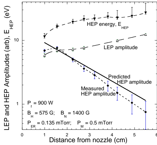
Figure 3: LEP and HEP amplitudes and HEP energy versus distance from the nozzle midplane. The model used to predict the HEP amplitude is based on plasma tied to field lines, the continuity equation, and metastable quenching by collisions with neutrals.
