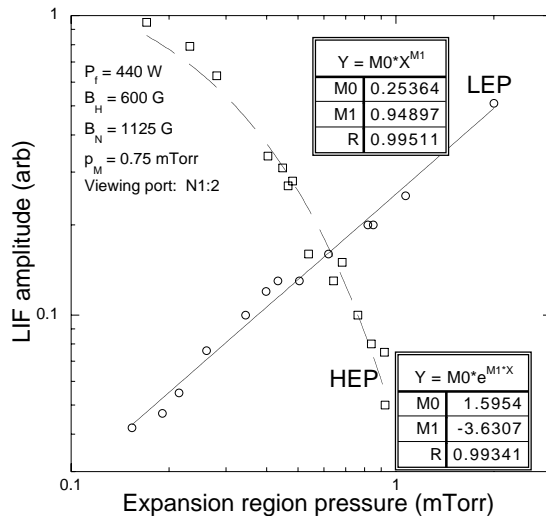
Figure 4: Dependence of HEP and LEP amplitudes on expansion region pressure at z = 2 cm in the ER.
