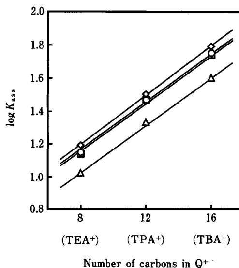
Fig. 8 Relationships between the ion association constants and carbon number of Q + . ○, AD-1; △, AD-2; □, AD-3; ◇, AD-4.
