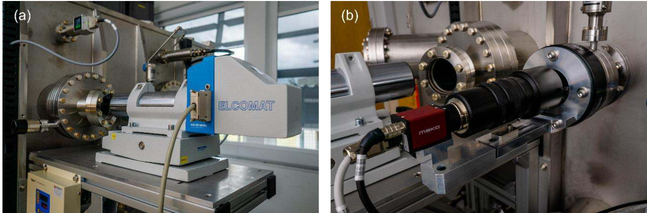
Figure 4: (a) An Elcomat3000 autocollimator is mounted to the system for in-situ metrology of the test mirror. (b) A Mako-G camera system will be used for alignment of the workpiece relative to the position of the ion beam.
