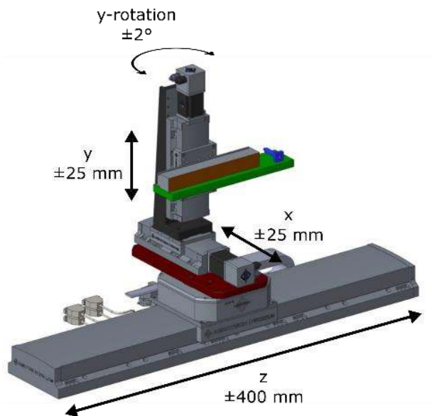
Figure 3: A 4-axis in-vacuum motion stage system is used to manipulate the workpiece.
