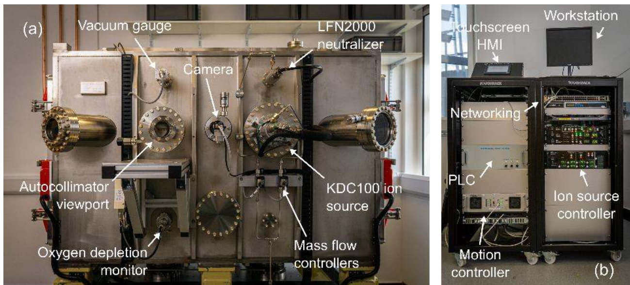
Figure 5: Photographs of (a) the IBF vacuum vessel and (b) control rack in the IBF lab at DLS. The vessel and the rack are connected by a set of modular cables which allows for easy connection and disconnection when the system is transported.
