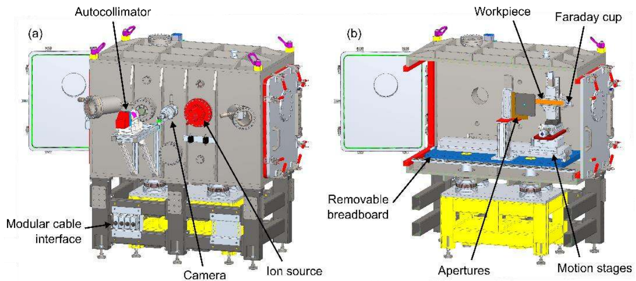
Figure 1: 3D model of IBF system designed and built at DLS. (a) Ion source, camera, and autocollimator are mounted externally on the vacuum vessel. (b) In-vacuum components, such as the motion stages and apertures, are mounted on a removable breadboard (highlighted in blue).
