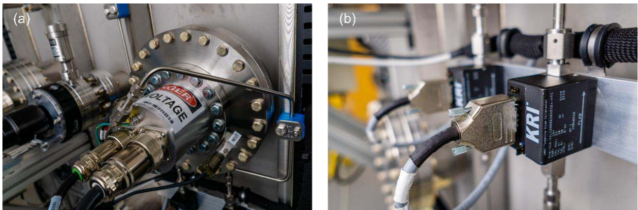
Figure 2: (a) The Ar ion beam is generated by a KRi KDC100 ion source. Apertures are used to select the size and shape of the ion beam incident upon the mirror being figured. (b) The flow rate of Ar gas supplied to the source and neutralizer can be set independently via mass flow controllers.
