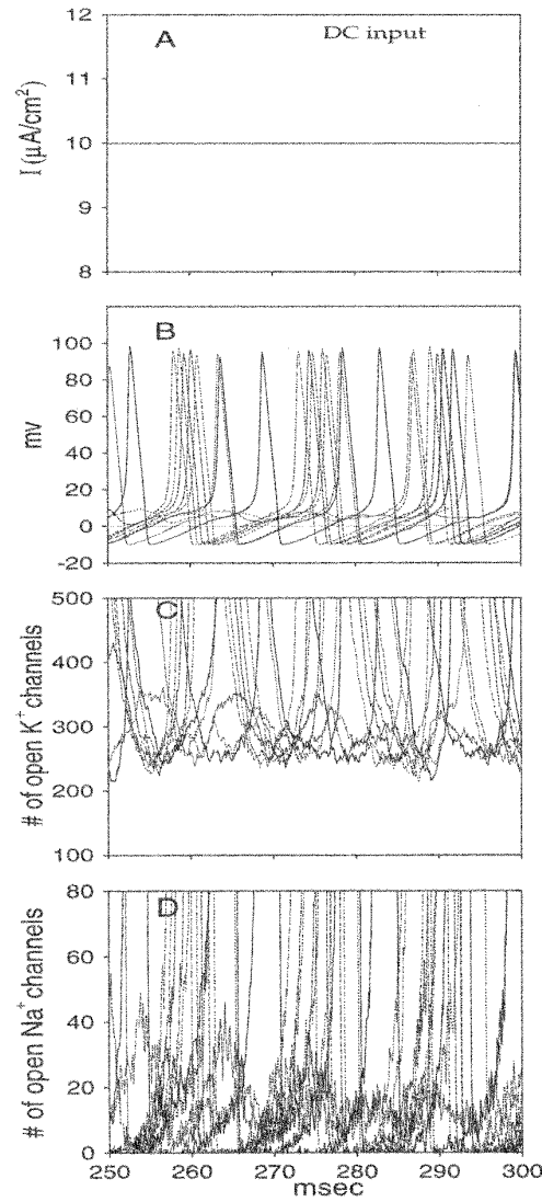
Figure 3: Channel fluctuations ruin the reliability of spike timing in the case of DC current input. (A) 10 \mu\text{A}/\text{cm}^2 DC current injected to a 600 \mu\text{m}^2 stochastic HH model (10,800 \text{K}^+ channels and 36,000 \text{Na}^+ channels) results with dispersed spike timings for repeated simulation (10 superimposed voltage traces) in B. (C, D) the number of open \text{Na}^+ and \text{K}^+ channels, respectively, corresponding to the voltage traces presented in B.
