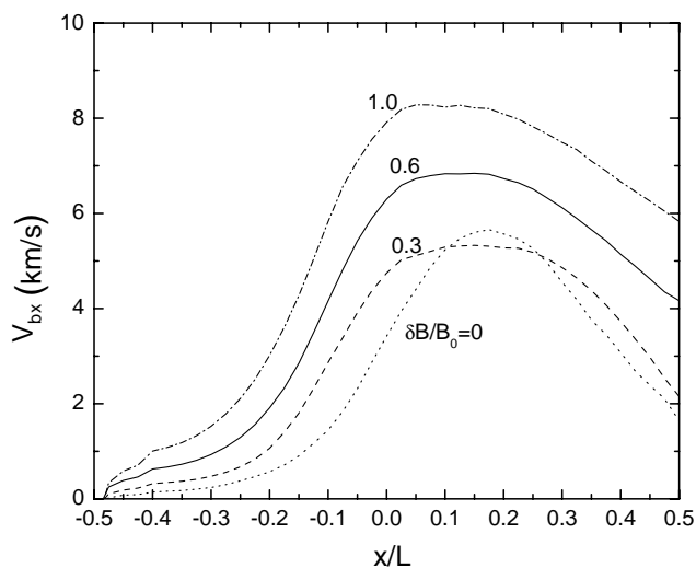
Fig. 7. Oxygen bulk velocity along x for different turbulence levels (as indicated).
