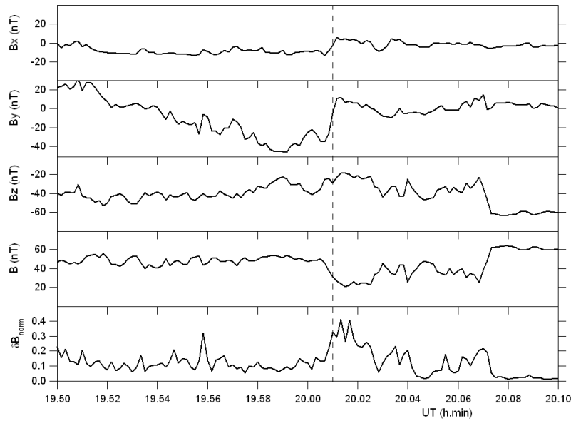
Fig. 1. Magnetic field components measured by the Cluster spacecraft during the 13 February 2001, magnetopause crossing, averaged over 10 s. From top to bottom, the three magnetic field components in the GSM system, the magnetic field magnitude, and the fluctuation level \delta B normalized to the local magnitude are shown. The simulation box of the numerical study corresponds approximately to the measurements going from 20:00:30 UT to 20:01:30 UT.
