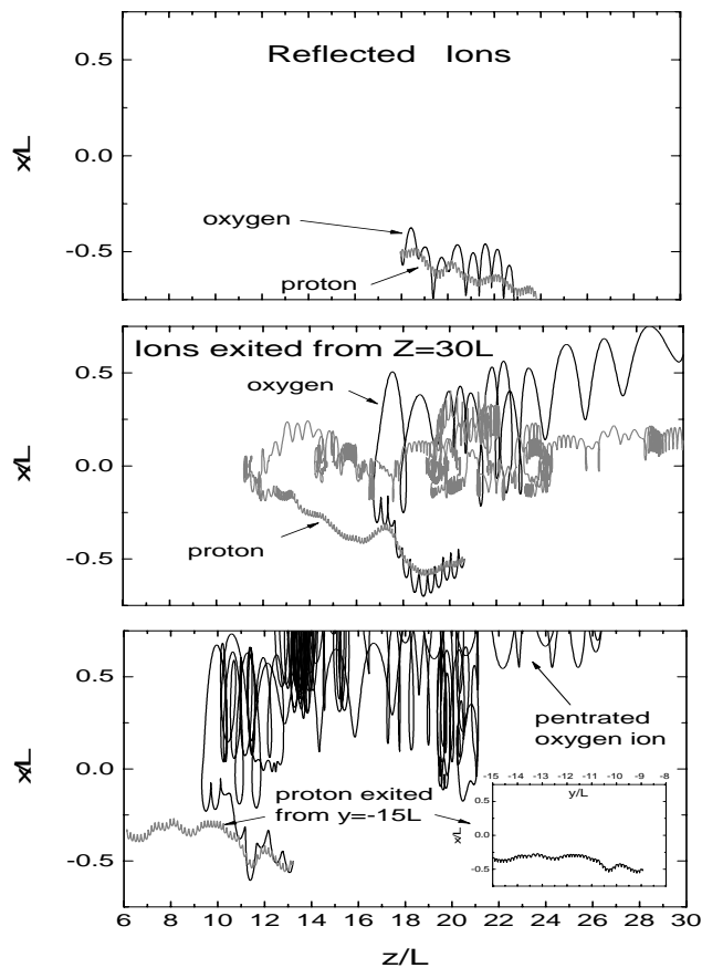
Fig. 2. Sample trajectories of proton and oxygen ions in the simulation box, for \delta B/B_0=0.6 . All the particles are injected at x=-0.5L . Black lines: oxygen. Grey lines: protons. Upper panel: particles exiting from the injection side (“reflected”). Middle panel: particles exiting from the side boundaries. Lower panel: oxygen exiting from the magnetosheath side, proton from the side boundaries.
