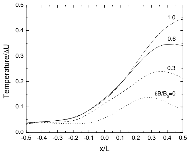
Fig. 9. Oxygen temperature profiles for different turbulence levels. Dimensionless units.
