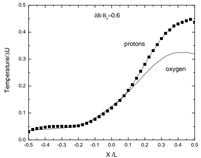
Fig. 5. Temperature profiles for proton and oxygen ions. Dimensionless units.
