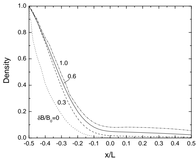
Fig. 6. Oxygen density profile for different turbulence levels (as indicated). Dimensionless units.
