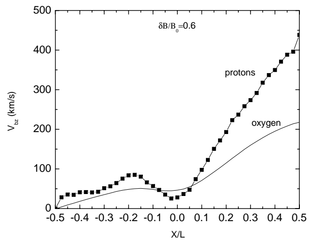
Fig. 4. Bulk velocity along z in the simulation box for proton and oxygen ions.
