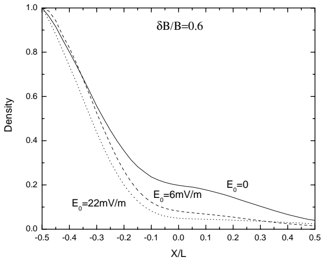
Fig. 10. Oxygen density profiles for different values of the electric field (as indicated). Dimensionless units.
