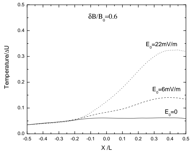
Fig. 12. Oxygen temperature profiles for different values of the electric field. Dimensionless units.
