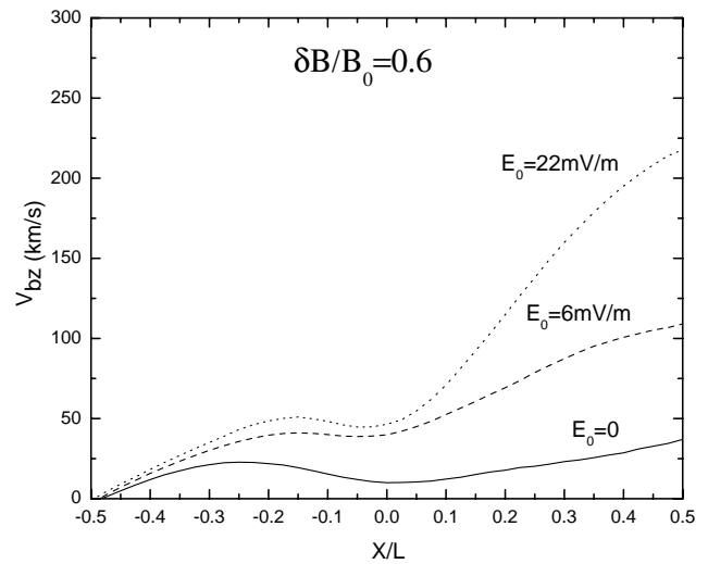
Fig. 11. Oxygen bulk velocity along z for different values of the electric field.
