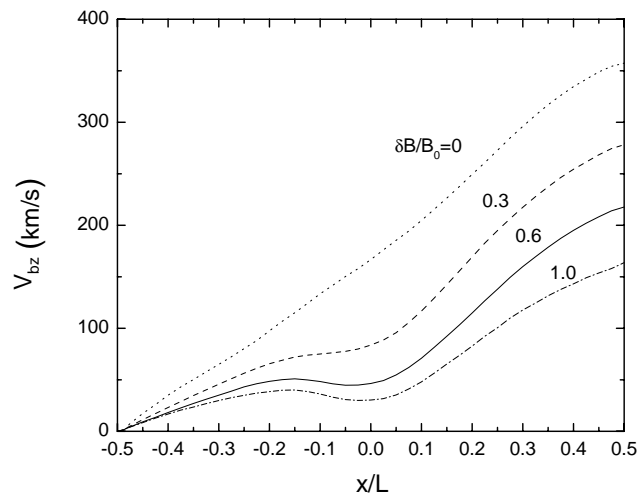
Fig. 8. Oxygen bulk velocity along z for different turbulence levels (as indicated).
