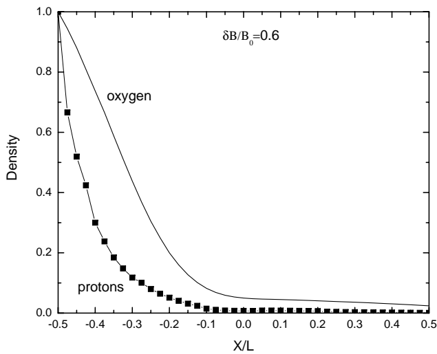
Fig. 3. Density profiles in the simulation box for proton and oxygen ions. Dimensionless units.
