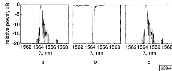
Fig. 4 Add/drop performance of filter
