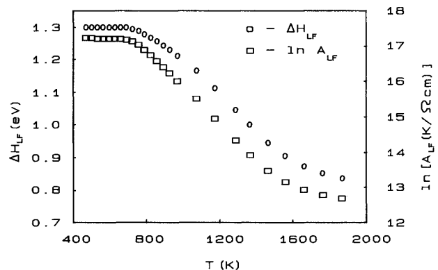
FIG. 2. Values of \Delta H_{LF} and A_{LF} obtained by the LF method vs absolute temperature.
