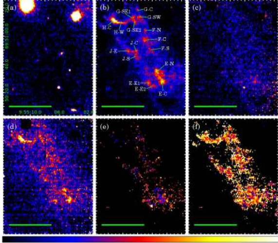
Figure 2. (a) Continuum surface brightness, (b) H\alpha intensity, (c) [N II]\lambda 6583 intensity, (d) [S II]\lambda\lambda 6716, 6731 intensity, (e) [N II]/H\alpha ratio, and (f) [S II]/H\alpha ratio maps of a part of the M82 cap. The color scales are 0-3.3 \times 10^{-19} \text{ erg cm}^{-2} \text{ s}^{-1} \text{ \AA}^{-1} ( 0.45 \text{ arcsec}^{-2} ), 0-2.5 \times 10^{-17} \text{ erg cm}^{-2} \text{ s}^{-1} ( 0.45 \text{ arcsec}^{-2} ), 0-1.5 \times 10^{-17} \text{ erg cm}^{-2} \text{ s}^{-1} ( 0.45 \text{ arcsec}^{-2} ), 0-1.0 , and 0-1.0 for the continuum, H\alpha , [N II] , [S II] , [N II]/H\alpha , and [S II]/H\alpha maps, respectively. Two bright stars appeared at upper side in the panel (a) are masked in the panels (b)–(f). North is up and east is left. Bar in lower left in each panel represents 30'' , which corresponds to 0.5 \text{ kpc} . Knot IDs are displayed in the H\alpha intensity map. (A color version of this figure is available in the online journal.)
