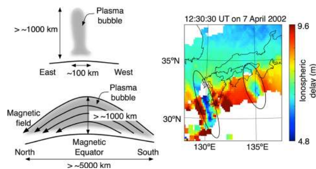
Fig. 1 General features of plasma bubbles. Left cross sections of plasma bubble in a zonal-vertical plane over the magnetic equator ( top ) and in a meridional-vertical plane ( bottom ) are illustrated. Right an example of plasma bubbles seen on an ionospheric delay map is also shown. Two ovals indicate plasma bubbles
