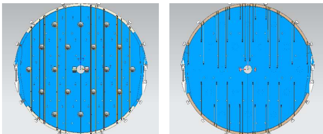
Figure 11. Left: front view of the anti-rotation ribbons and mirrors support cones. Right: rear view of the stabilizing ribbons.
