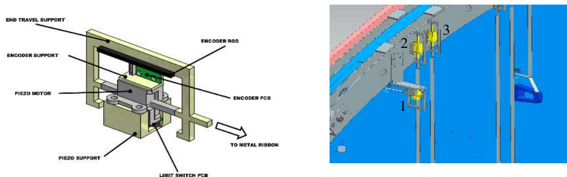
Figure 15. Left: view of a piezo-electric motor. Right: view of three piezo-electric motors (in yellow) on the frame. Motors 2 and 3 are oriented vertically and use the transmission tool (one connected to a different motor is shown in blue), while motor 1 is oriented horizontally and is directly connected to the mirror.
