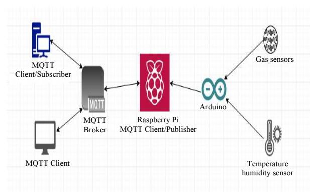
Fig. 1: Proposed Architecture for IOT Based GHMS
