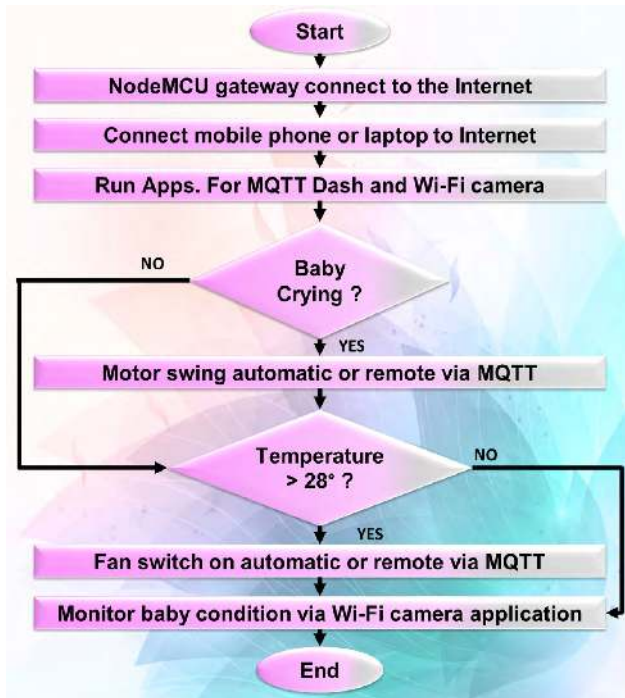
FIGURE 15. Flowchart of the system.
