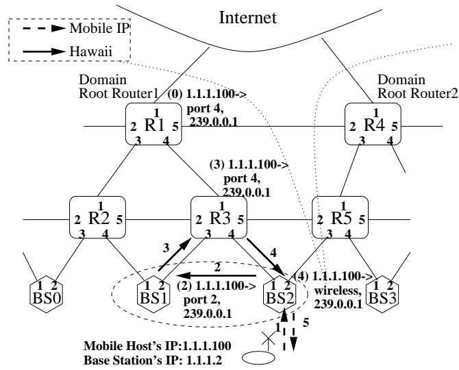
Figure 4: Intra-domain handoff
