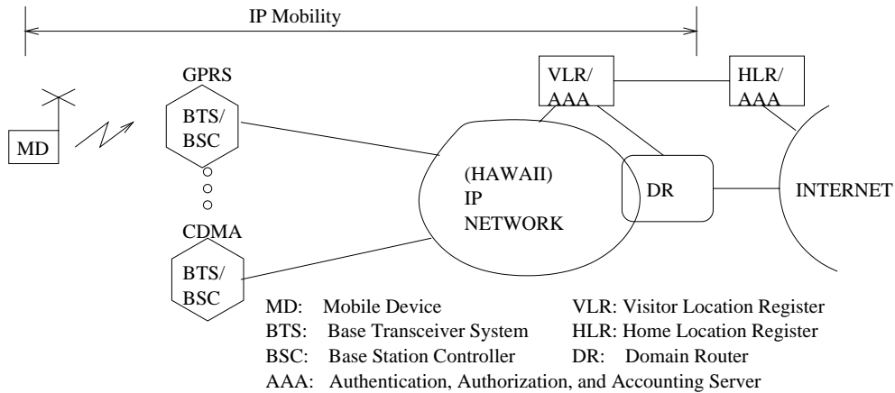
Figure 8: HAWAII-based architecture
