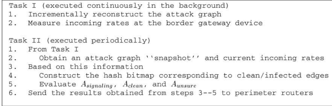
Fig. 7. Attack Mitigation Decision-making (AMD) algorithm.
