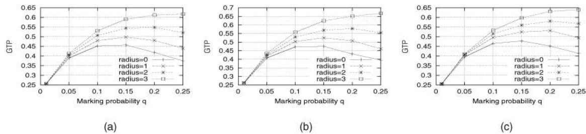
Fig. 14. GTP (Good Traffic Percentage) by increasing perimeter radius.
