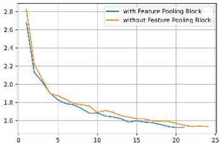
Figure 7: Convergence performance
