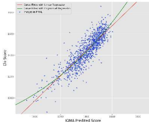
Figure 6: IQMA predicted scores vs. Elo scores on PIPAL validation set.
