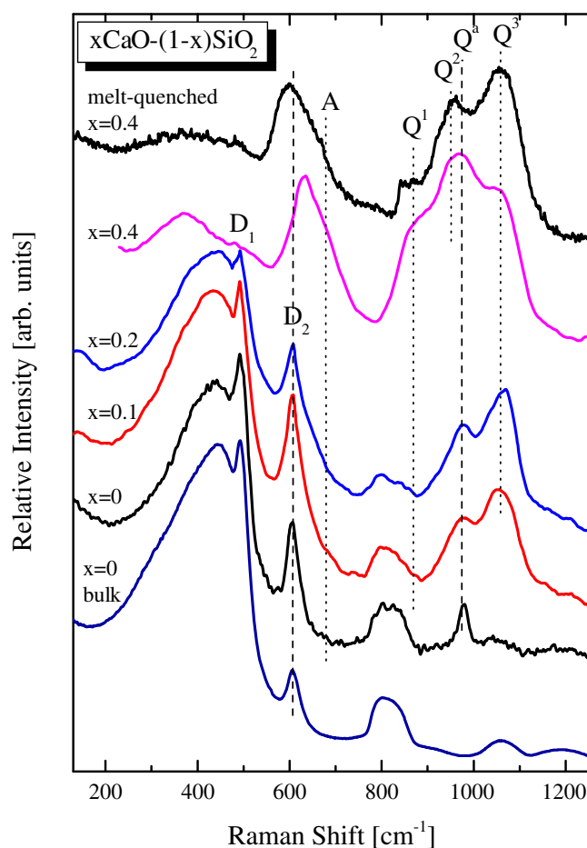
Figure 2. Representative Stokes-side Raman spectra of x\text{CaO}-(1-x)\text{SiO}_2 ( x = 0, 0.1, 0.2 and 0.4 ) glasses prepared by sol-gel technique at room temperature. The Raman spectra of the bulk, melt-quenched \text{SiO}_2 and the 0.4\text{CaO} \cdot 0.6\text{SiO}_2 glasses are also shown at the bottom and top of this figure, respectively.
