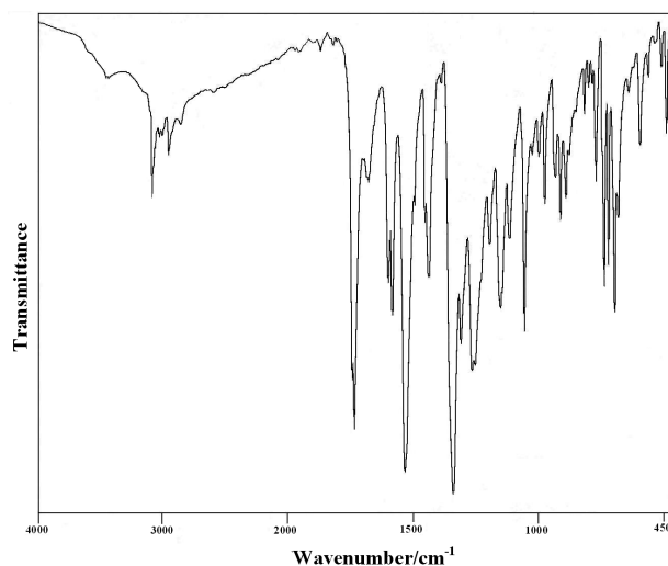
Figure 1. IR spectrum.
