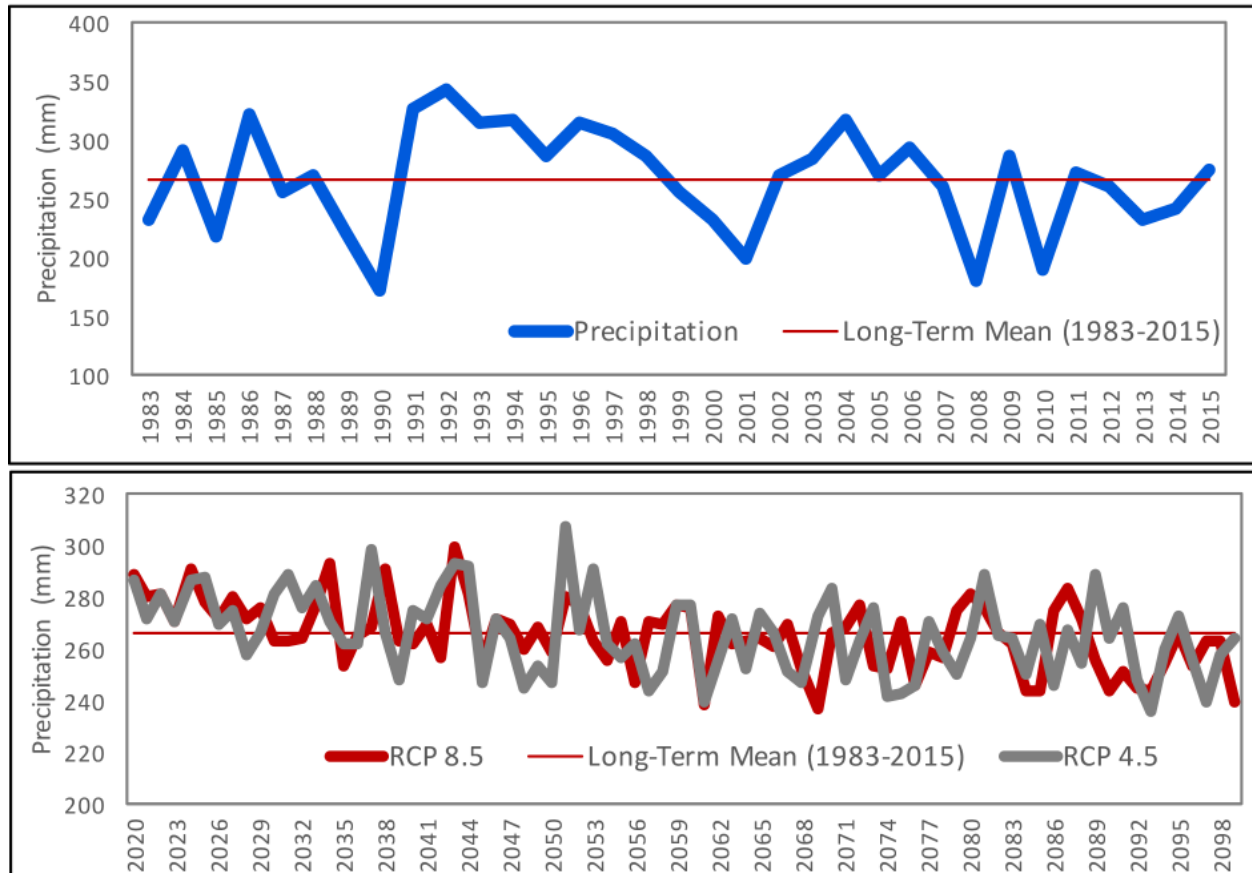
Figure 2- (Top) Satellite-based observed annual precipitation 1983-2015; (Bottom) Precipitation projections based on ensemble means of multiple climate model simulations under two Representative Concentration Pathways 4.5 and 8.5 (source: http://rainsphere.eng.uci.edu/ ).
