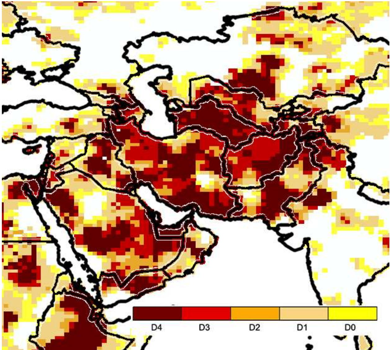
Figure 1- Spatial patterns of drought in mid-2000 based on the Multivariate Standardized Drought Index (MSDI 43 ). Most of Iran was in Extreme and Exceptional drought (D0: Abnormally Dry ; D1: Moderate Drought; D2: Severe Drought; D3: Extreme Drought; D4: Exceptional Drought).
