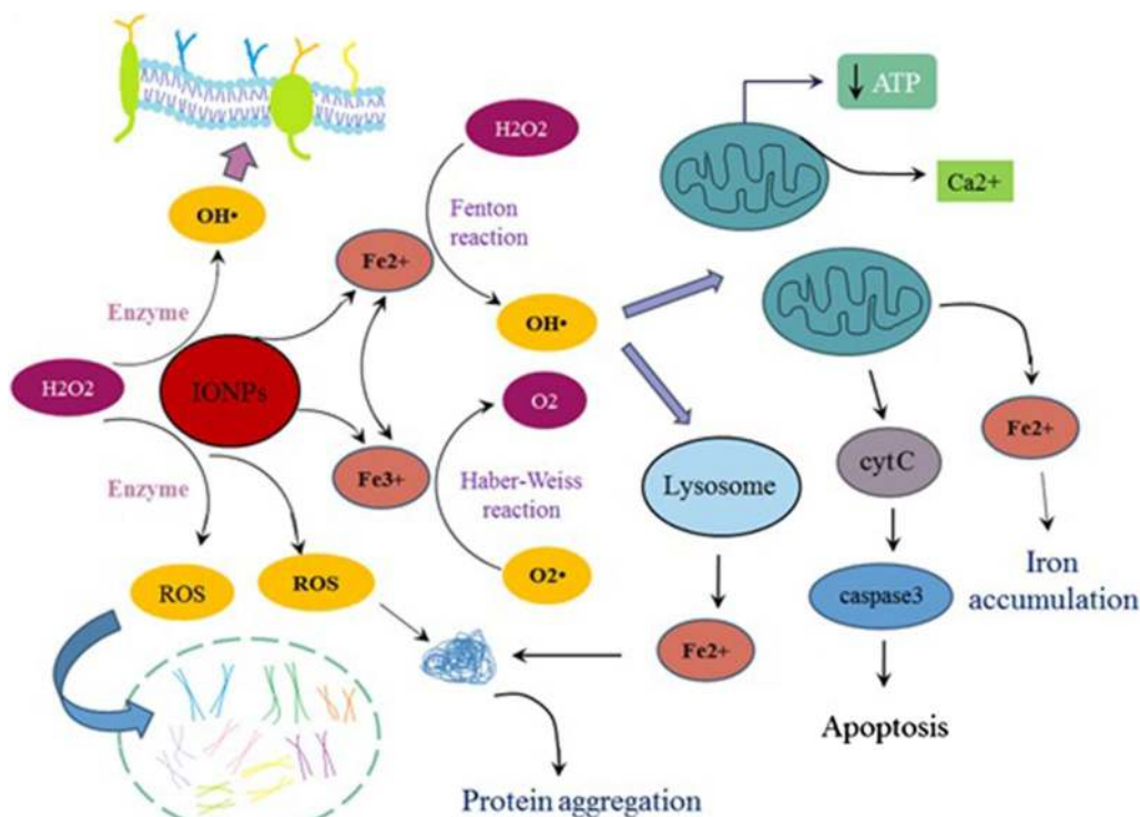
Fig. 1 IONPs can cause iron accumulation, oxidative stress, and protein aggregation. IONPs present a large surface area for redox cycling [9]; in addition, the iron ions released from IONPs can also contribute to Fenton's reaction, produce OH^\bullet from H_2O_2 , and finally lead to oxidative stress [57]. Reactive oxygen species (ROS) may directly damage DNA, cell membrane, and organelle's membrane. ROS result in release of Ca^{2+} and cytochrome C from mitochondria, and therefore, induction of apoptosis [11]. Furthermore, ROS leads to the release of iron from lysosomes and mitochondria through damaging organelle's membrane, [18], and iron accumulation in cytosol. Both ROS and free iron interact with a number of proteins, change their conformation, and mediate their aggregation [25]
