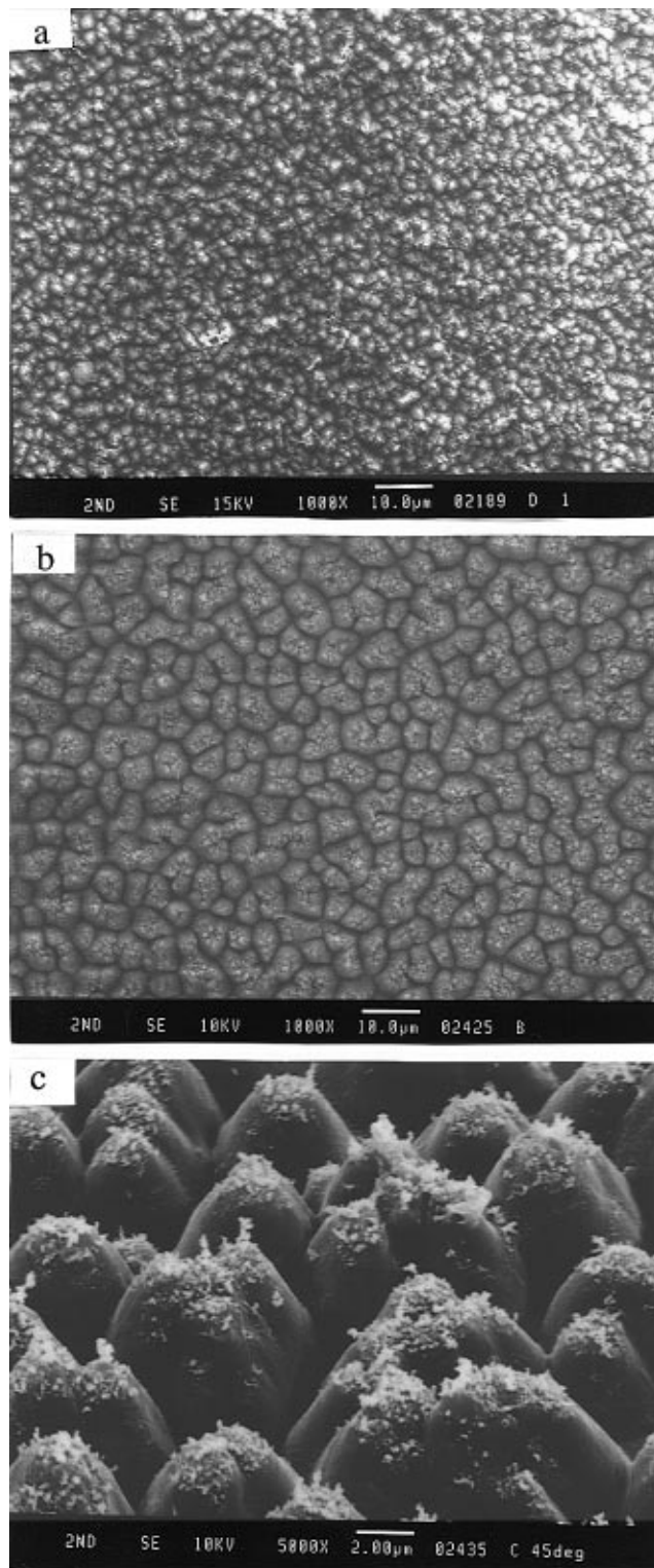
Figure 3. Scanning electron micrographs of surface changes: (a) after 10 pulses with 36 \text{ mJ cm}^{-2} at 248 nm; (b) after 250 pulses with 36 \text{ mJ cm}^{-2} at 248 nm; (c) enlarged view of (b) at 45^\circ .
