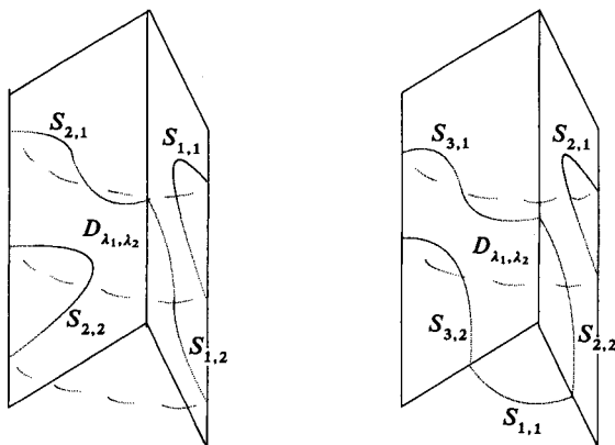
FIGURE 6. The disks for the 3-ended and 4-ended Costa surfaces.
